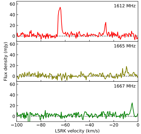
Figure 1. Spectrum of G341.2969+0.3504.
