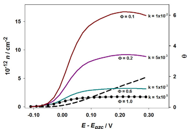
Fig. 5. Particle number density (left) and effective coverage (right) at the liquid/liquid boundary as a function of applied potential estimated from photocurrent responses assuming various values of k_2 (denoted in the graph). Trends estimated from interfacial capacitance (dashed black line) and assuming a perfect quantum yield (Eq. (9), solid circles) are also shown. This analysis is based on data obtained in the presence of Fc, [\text{TiO}_2] = 400 \text{ mg L}^{-1} and I_0 = 4.7 \times 10^{14} \text{ cm}^{-2} \text{ s}^{-1} .
