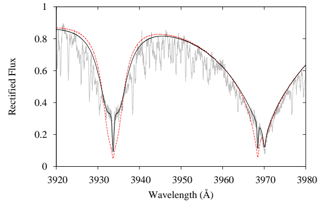
Figure 7. The Ca H and K lines in the FIES spectrum (grey line) taken on 2013 August 6 shows the distinctive pointed core due to element stratification. The solid line shows a synthetic line profile created using a step-shaped stratified abundance profile, while the red dashed-line shows a normal non-stratified synthesis.
