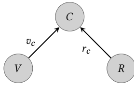
Figure 3: Criticality class (C) with associated classes Vulnerability (V) and Risk (R) and object properties vulCriticality ( vc ) and riskCriticality ( rc )
