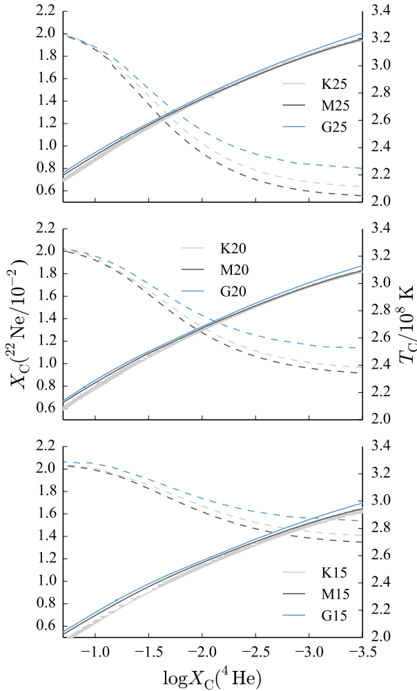
Figure 10. Central ^{22}\text{Ne} abundances (dashed lines) and central temperatures (solid lines) during the core helium-burning phase.
