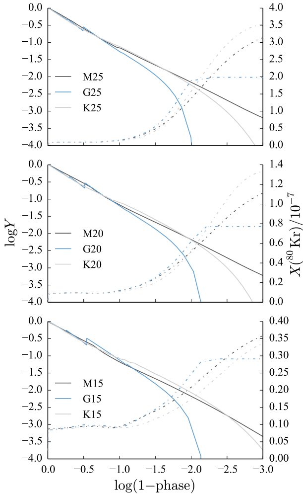
Figure 9. Central {}^4\text{He} (solid lines) and {}^{80}\text{Kr} ( s -only; dot-dashed lines) abundances during the core helium-burning phase. The x -axis is \log(1 - \text{phase}) , where phase = 0 at helium ignition (left side of the plot) and 1 at helium depletion (right side of the plot).
