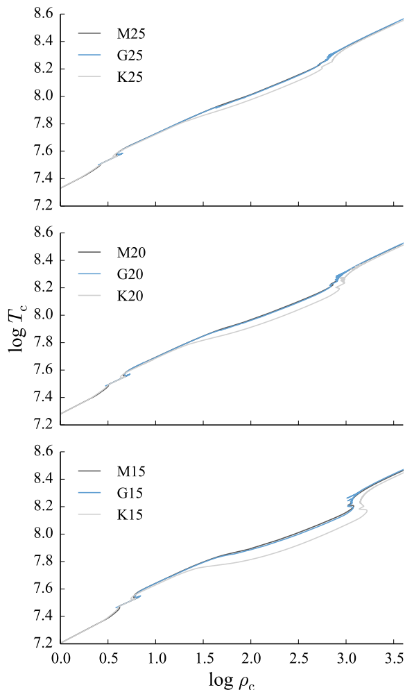
Figure 3. Evolution of the central temperature and density during the core hydrogen- and helium-burning phases.
