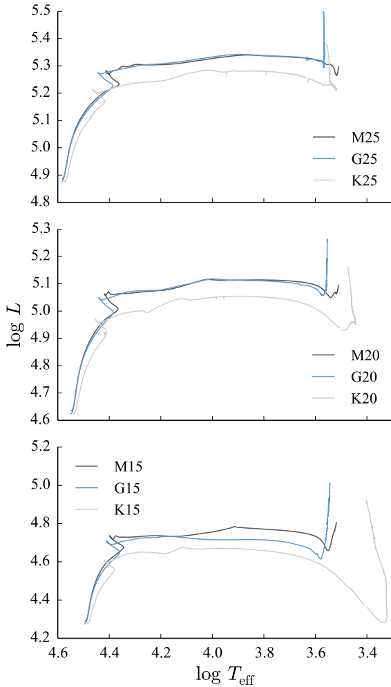
Figure 2. Evolution of the models in the Hertzsprung-Russell (H-R) diagram.
