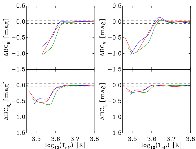
Figure 3. Model-dependent corrections ( \Delta BC , defined as BC_{\text{empirical}} - BC_{\text{theoretical}} ) calculated as a function of T_{\text{eff}} for the optical BV(RI)_c Johnson–Cousins bandpasses. Corrections are shown for the following models: BCAH98 \alpha = 1.9 (red), DCJ08 (blue) and updated Pisa (green). The dashed lines represent the \pm 0.05 mag level with respect to zero.
