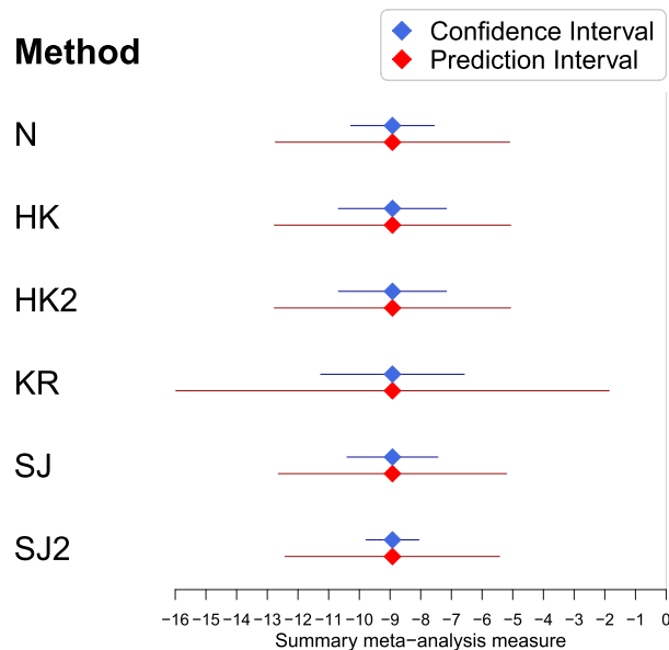
Figure 6. The summary results for the post-treatment difference in diastolic blood pressure between the treatment and control groups based on a random effects meta-analysis fit using restricted maximum likelihood with confidence and prediction intervals constructed using a variety of methods. N, conventional method; HK, Hartung-Knapp; HK2, modified Hartung-Knapp; KR, Kenward-Roger; SJ, Siddik-Jonkman; SJ2, modified Sidik-Jonkman.
