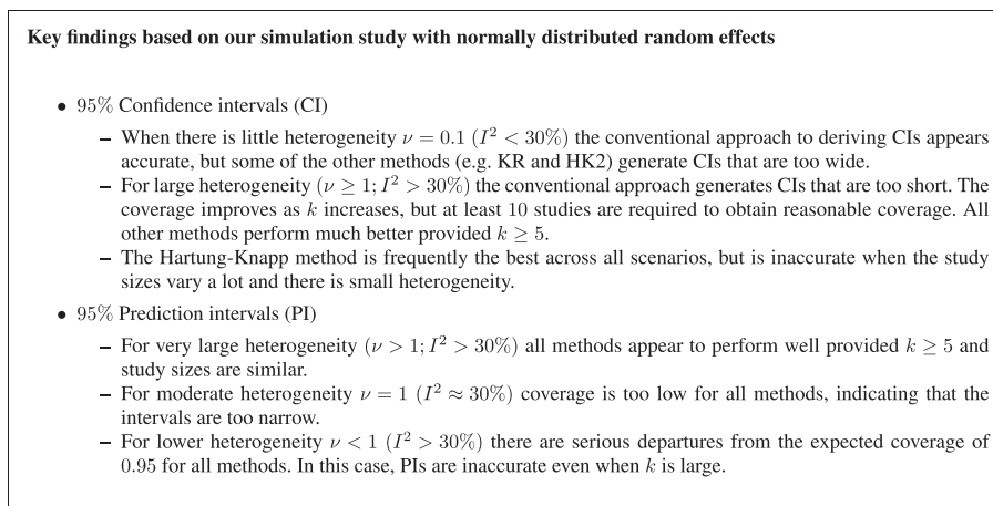
Figure 7. Key findings regarding the coverage performance of confidence intervals (CIs) and prediction intervals (PIs) obtained using the conventional and modified intervals for a random-effects meta-analysis model (1) with estimation via restricted maximum likelihood.
