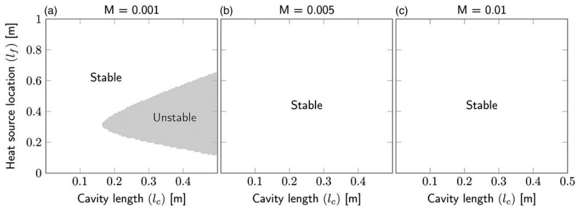
Figure 15. Stability maps for mode I and different Mach numbers (a) M = 0.001 , (b) M = 0.005 and (c) M = 0.01 , for a combustor with T_1 = T_2 = 288 K.
