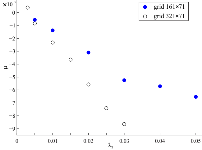
FIG. 2. Non-Gaussianity as measured by \mu , the ratio of statistically averaged nonlinear and linear energy as function of the coarse-graining parameter \lambda_k . \mu is averaged over 600 characteristic periods of the final stage of evolution before the spectral peak reaches k_p = 1 .
