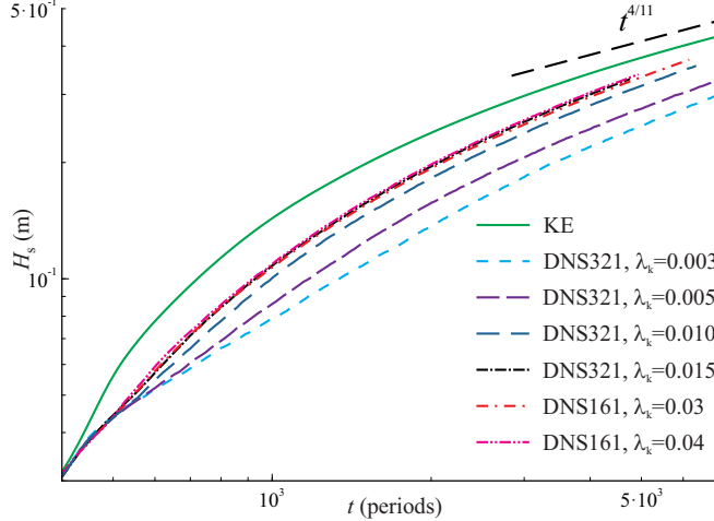
FIG. 4. Evolution of significant wave height H_s : DNS on 161 \times 71 and 321 \times 71 grids for different values of \lambda_k vs the KE simulation
