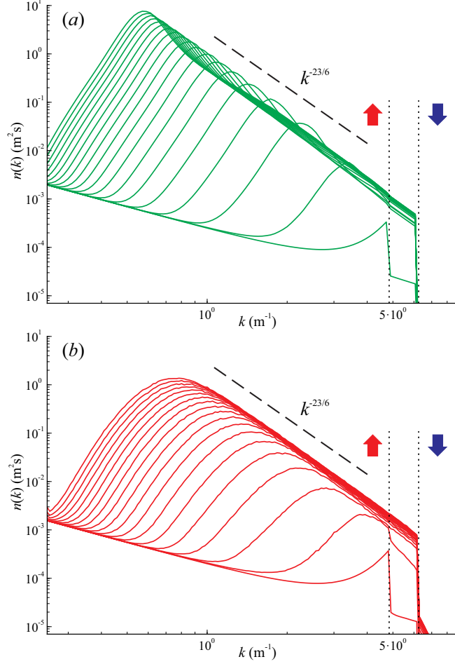
FIG. 1. Development of wave action spectrum n(k) under the constant wind U = 2c_1 , shown in steps of approximately 300\tau_1 , where c_1 and \tau_1 are characteristic phase speed and period, corresponding to k = 1 . (a) KE, WRT algorithm (b) DNS, with \lambda_k = 0.03 on 161 \times 71 grid. Wavenumber ranges of forcing and dissipation are indicated by arrows
