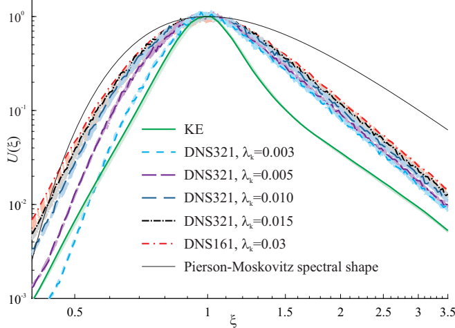
FIG. 3. Self-similar shape function \mathcal{U}(\xi) , \xi = kt^{6/11} , extracted from the numerical solutions at the last 1000 wave periods of evolution. Shapes at every 100 periods are shown in light colours, the final curve is in darker colour of the same hue, normalized for \mathcal{U}(1) = 1 . Numerical models used are the KE and the DNS on 161 \times 71 (DNS161) and 321 \times 71 (DNS321) grids for different values of \lambda_k
