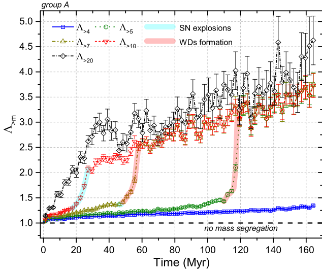
Figure 1. \Lambda_{>m} parameter, as a function of time (in Myr), for the simulations of group A. The dashed black line at \Lambda_{>m} = 1 indicates the absence of mass segregation. Solid blue line (with squares): stars with mass m > 4M_{\odot} . Dotted green line (with circles): stars with m > 5M_{\odot} . Dash-dot-dot dark yellow line (with upward triangles): stars with m > 7M_{\odot} . Dashed red line (with downward triangles): stars with m > 10M_{\odot} . Dash-dot black line (with rhombi): stars with m > 20M_{\odot} . The thick, semi-transparent cyan and red lines highlight the intervals in which SN explosions and the formation of WDs, respectively, occur. Here, m does not refer to the initial mass of a star, but to its mass at the time shown on the x -axis.
