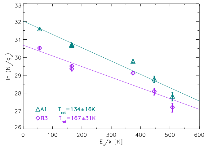
Figure 4. Rotational diagram of CH 3 OH detected toward A1 and B3. The results of the rotational diagram analysis were used as the initial parameters for the MADCUBAUJ modeling.
