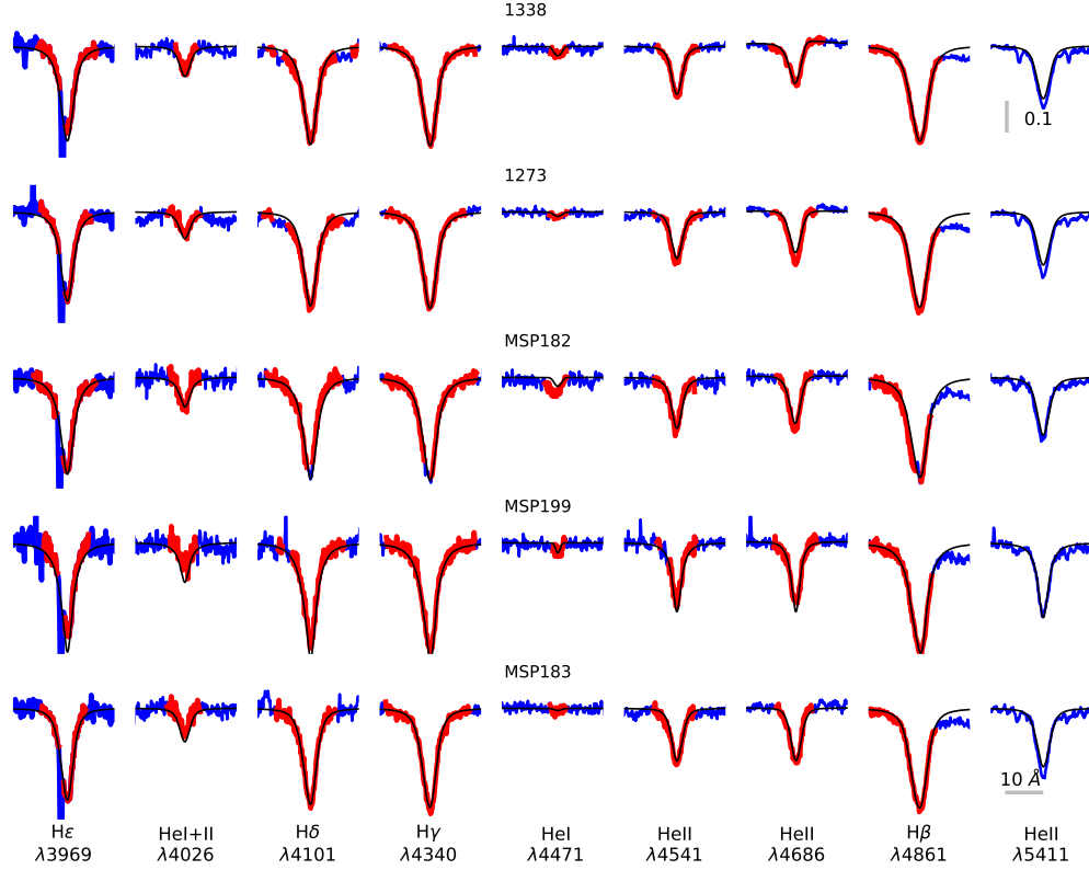
Figure 3. Final fits to the observed target and control stars. We represent in red the part of the observed spectra that has been used for the analysis, in blue parts of the observed spectra not used for the analysis and in black the theoretical spectra, convolved with the rotational and macroturbulent velocities and the instrumental profile (assumed gaussian). The gray horizontal and vertical lines give the axes scales
