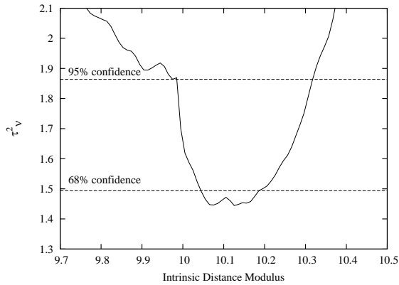
Figure 10. \tau_r^2 as a function of distance for the fit to the 10 Myr Geneva isochrone. The 68 and 95 per cent confidence levels are marked.
