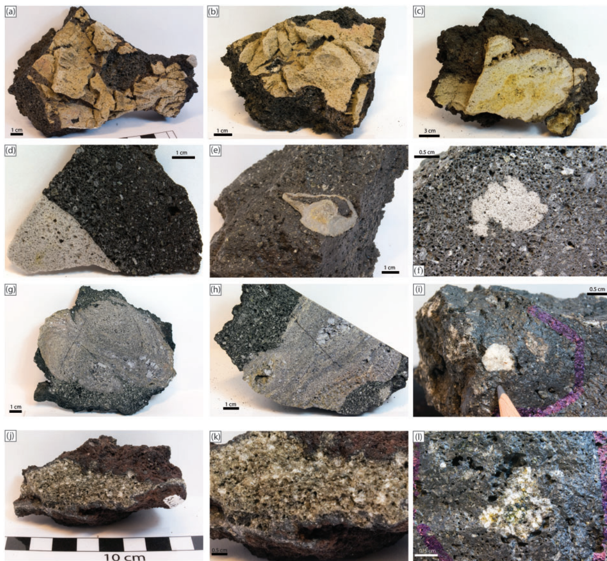
Fig. 2. Types of common xenolith in Anak Krakatau lavas. (a–c) Fragments of larger cream to grey-coloured, frothy, metapelitic xenoliths ('xeno-pumices') that are common in Anak products. (d–f) Small-scale features of frothy metasedimentary xenoliths. (Note the ductile shape of some smaller xenolith fragments, pointing towards xenolith disintegration in a hot and plastic state.) (g, h) Banded frothy xenolith with plastic deformation features (e.g. folding) and larger aggregates of pyro-metamorphic minerals such as cordierite [e.g. in (h), just top right of centre]. (i) Isolated cordierite xenocryst in Anak lava, testifying to the complete disintegration of some xenoliths. (j, k) Crystalline xenolith with frothy texture and glassy margin, probably of dioritic provenance, that is intensely strung out; (k) is close-up view of (j). (l) Small fragment of gabbroic composition in Anak lava.
