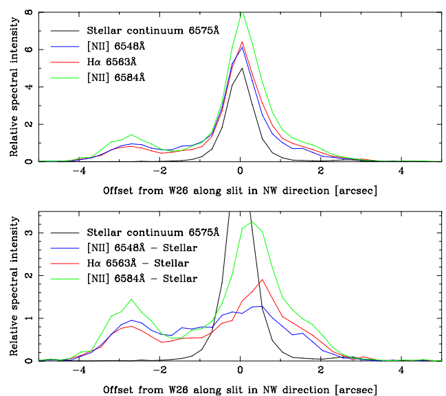
Figure 4. Spatially resolved emission along the VLT/FORS slit (as shown in Fig. 2) at the [N II] 6548, 6584 and H \alpha emission lines, as well as at 6575 Å to show the stellar continuum emission. The upper panel shows absolute measurements while the lower panel shows the emission lines with the stellar continuum subtracted (as well as the stellar continuum profile itself for reference).
