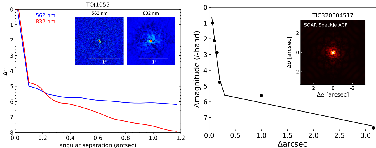
Figure 3. Left panel: Zorro speckle imaging and 5\sigma contrast curves of HD 183579 at 562 nm and 832. The data reveal that no companion star is detected within the spatial limits of 1 AU out to 57 AU with a \Delta m of 5 to 8. Right panel: Speckle ACF obtained in the I band using SOAR. The 5\sigma contrast curve for HD 183579 is shown by the black points. Black solid line corresponds to the linear fit of the data, at separations smaller and larger than \sim 0.2 arcsec.
