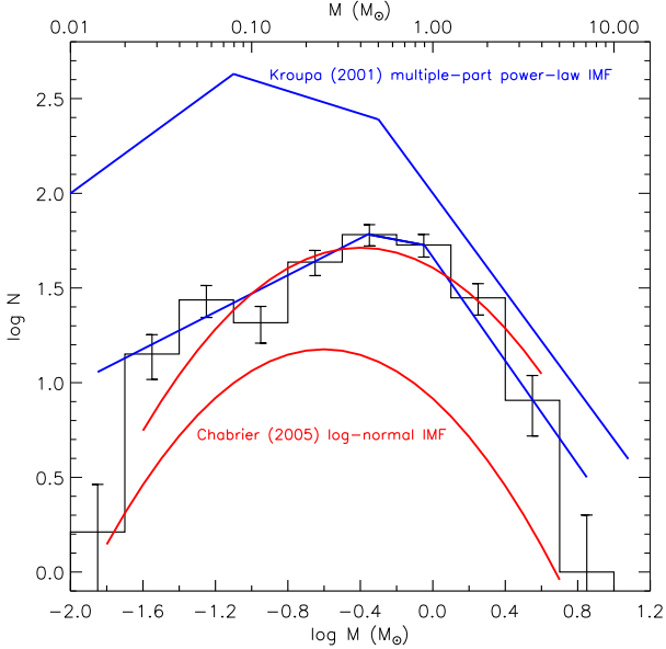
Figure 11. Comparison of the IMF of NGC 6611 with well known theoretical functional forms: the multiple-part power-law IMF (labelled blue line, Kroupa 2001) and the log-normal IMF (labelled red line, Chabrier 2005). We have fitted such functions to the observed IMF (ignoring the two extreme bins); the most adequate fits are overplotted on the IMF. Both when compared to the power-law and log-normal formulations, the NGC 6611 IMF peaks at a slightly higher mass, \sim 0.45 M_{\odot} (see text).
