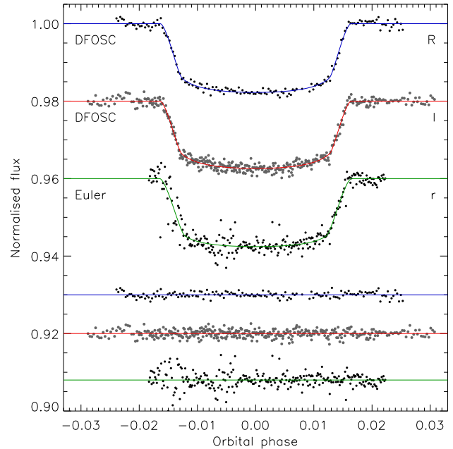
Figure 6. As Fig. 3, but for WASP-55.
