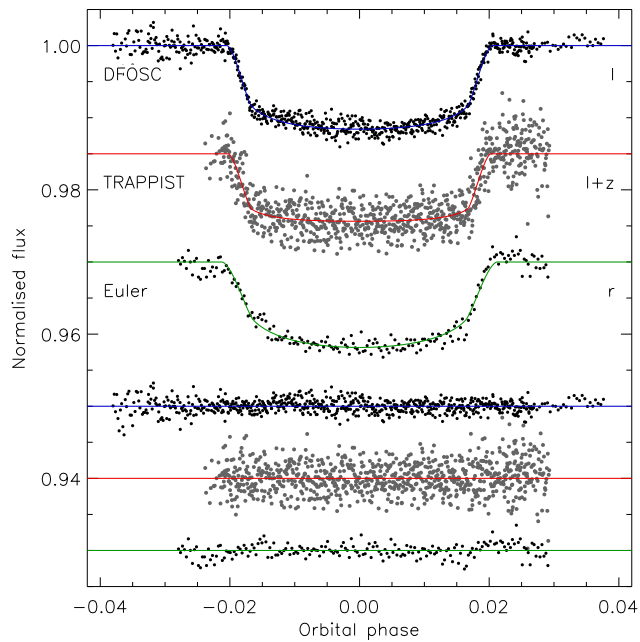
Figure 3. The phased light curves of WASP-22 analysed in this work, compared to the \text{JKTEBOP} best fits. The residuals of the fits are plotted at the base of the figure, offset from unity. Labels give the source and passband for each data set. The polynomial baseline functions have been subtracted from the data before plotting.
