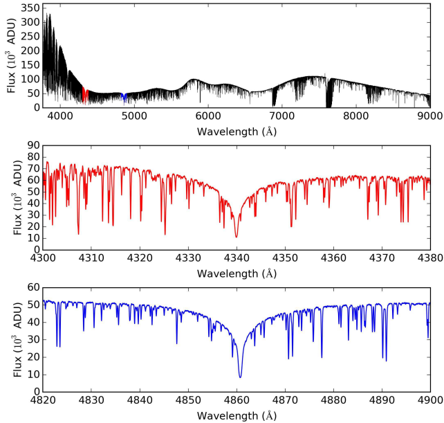
Figure 5. High-resolution spectrum of \theta Cyg taken with HERMES Mercator spectrograph in May 2011 (top), and region around H \gamma (middle) and H \beta (bottom).
