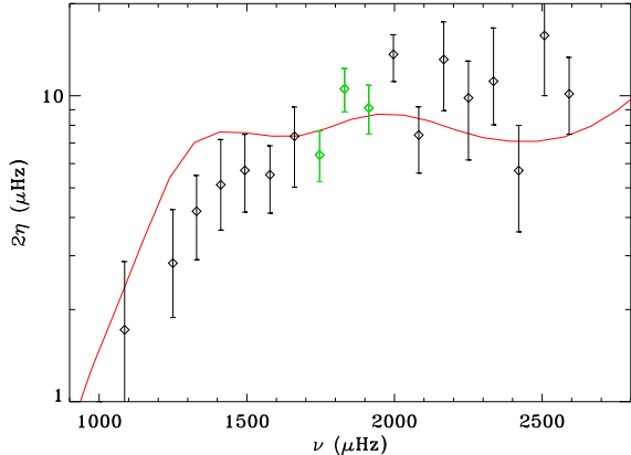
Figure 9. Twice the theoretical linear damping rates for radial modes as a function of frequency calculated for AMP Model 1 (Table 3) with mass M = 1.39 M_{\odot} , luminosity L = 4.215 L_{\odot} , effective temperature T_{\text{eff}} = 6753 K, and helium and heavy-element abundances by mass X = 0.7055 and Z = 0.01845 (solid red line). The diamond symbols show the measured linewidths for observed radial modes of Table 2, with 3\sigma error bars. The green symbols indicate the three most prominent consecutive modes.
