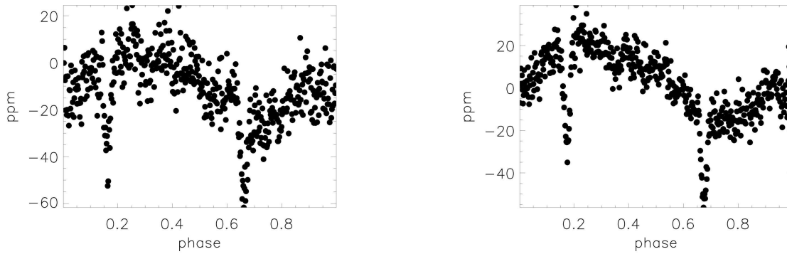
Figure 16. Q6 (left) and Q8 (right) light curve folded at 1.77627 \text{d}^{-1} ( \sim 20.56 \mu\text{Hz} ), showing that a faint background binary is the likely explanation for this frequency in the power spectrum.
