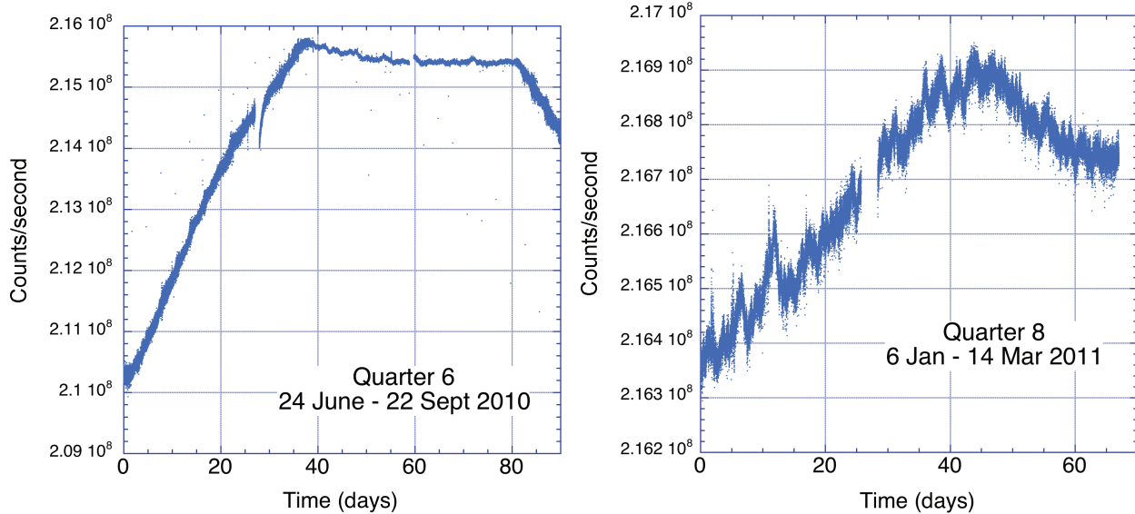
Figure 2. Kepler \theta Cyg unprocessed light curve for Quarter 6 (left) and Quarter 8 (right). The custom aperture captured the target completely in Q6 only during 42 d (flat portion of curve) used in this analysis. The spacecraft entered a safe mode for part of Q8, so only 67 days of data were obtained.
