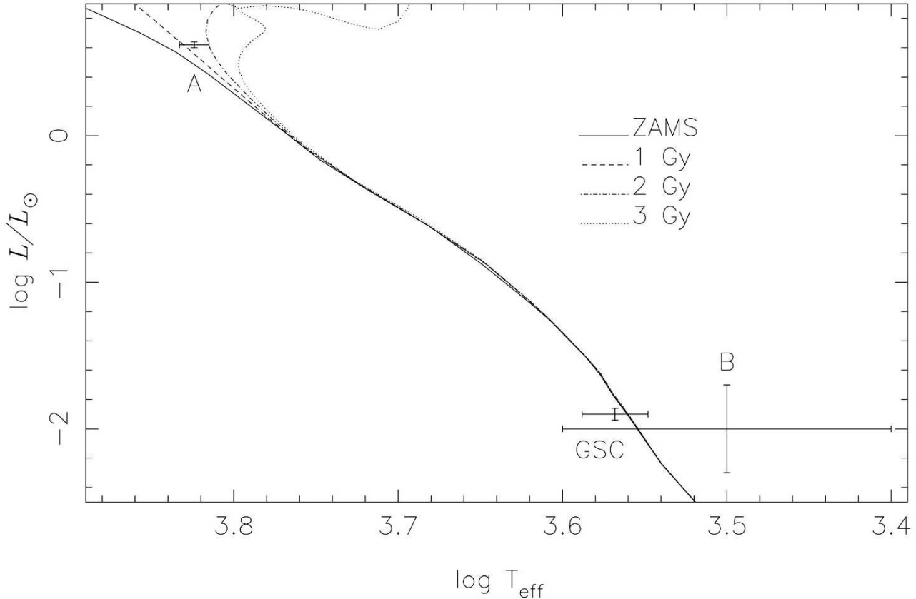
Figure A2. Hertzsprung-Russell diagram for \theta Cyg system, showing components A and B, plus the common proper-motion companion GSC 03564-00642. Models are from Marigo et al. (2008) .
