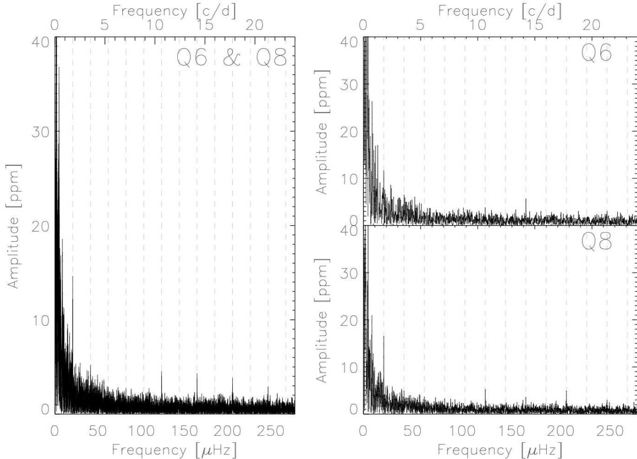
Figure 14. Fourier spectra of the individual quarters and the combined data, with the vertical dashed gray lines indicating the orbital frequency of the background binary and its harmonics. One remaining frequency at \sim 1.7 \text{ d}^{-1} probably is attributable to a background binary (see text and Fig. 16).
