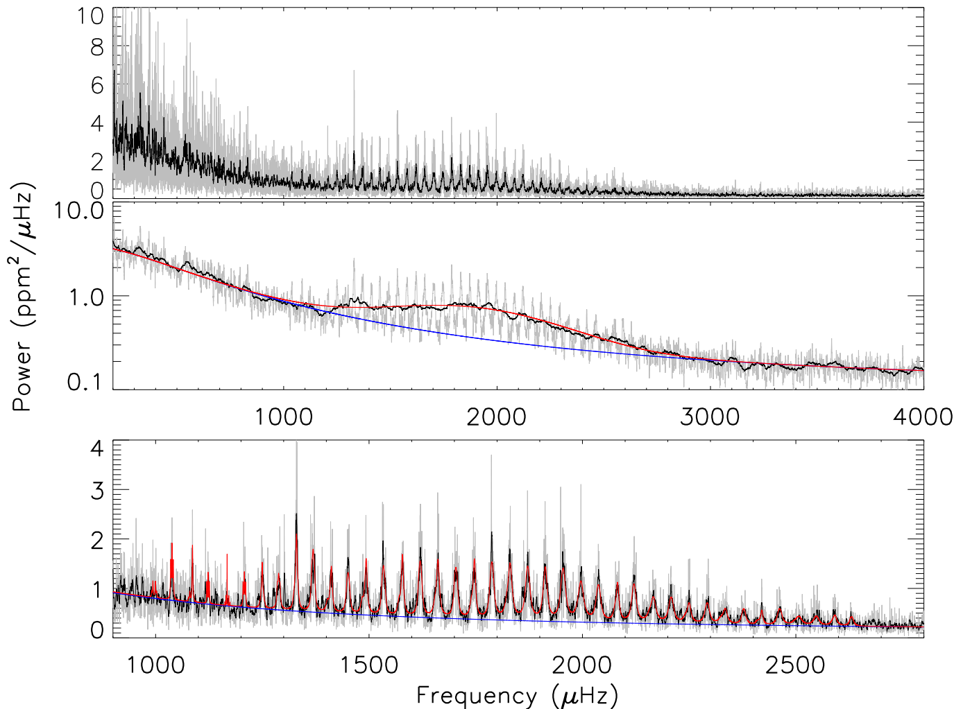
Figure 4. Top: Power-density spectrum of the Q6 and Q8 data shown using the minimally processed data (grey) and using a box-car smoothing of width 3 \mu\text{Hz} (black). Middle: Power spectrum with a smoothing of width 3 \mu\text{Hz} (grey) or \Delta\nu/2 = 42 \mu\text{Hz} (black). Superimposed is shown the best fit of the mode envelope with a Gaussian (red) and of the noise background (blue). Bottom: Zoom-in on the modes. The power spectrum is smoothed over 0.5 \mu\text{Hz} (grey) or 3 \mu\text{Hz} (black). The red curve shows the best fit to the individual pulsation modes with Lorentzian profiles.
