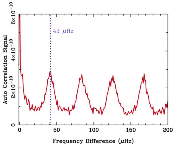
Figure 8. Autocorrelation of power spectrum, showing a 42- \mu\text{Hz} peak interpreted as half of the large frequency separation between modes.
