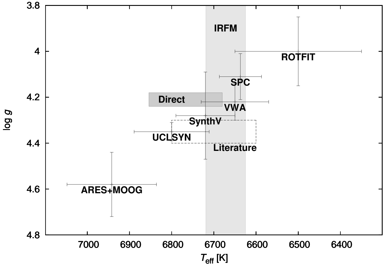
Figure 7. Comparisons of results from the analyses of HERMES and TRES spectra. The range of values of T_{\text{eff}} obtained by Blackwell & Lynas-Gray (1998) using the IRFM is shown by the light grey band. The interferometric T_{\text{eff}} from Ligi et al. (2012) and the asteroseismic \log g value are given as the dark grey box labelled ‘Direct’. The dashed box indicates the most-probable parameters from the literature review.
