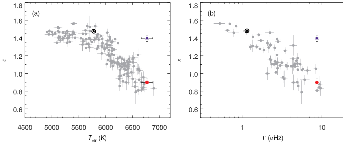
Figure 11. The possible locations of \theta Cyg (blue triangles for Scenario A and red circles for Scenario B) in the (a) \varepsilon - T_{\text{eff}} plane and (b) \varepsilon - \Gamma plane. Grey points are Kepler stars from White et al. (2012). The Sun is marked by its usual symbol. This figure shows that Scenario B is the more likely of the two discussed in Section 7, since an \varepsilon value of \sim 0.9 (as opposed to \sim 1.4 ) for \theta Cyg places it in line with the other Kepler stars.
