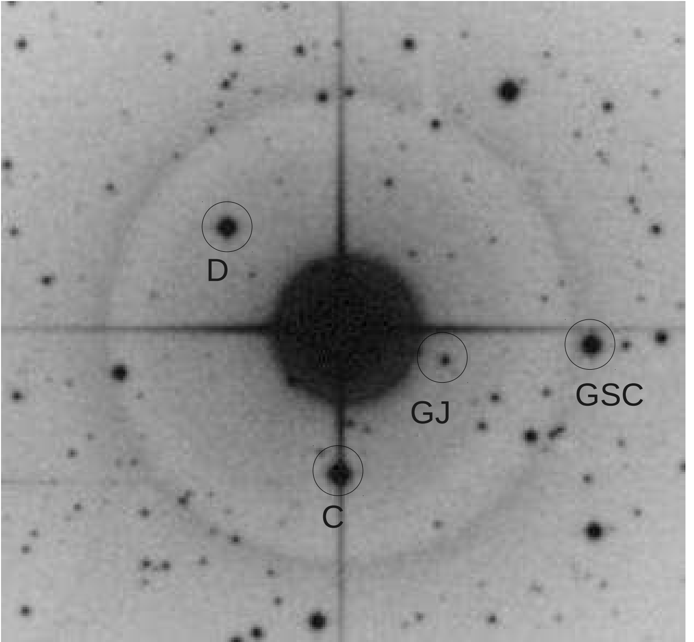
Figure A1. Digitized Sky Survey image showing the field around \theta Cyg AB. The scale of this figure is approximately 5\frac{1}{4} arc minutes wide. The stars discussed in the text are highlighted. GJ is GJ765B and GSC is GSC 03564-00642.
