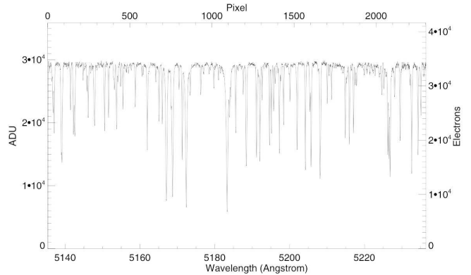
Figure 6. A spectrum of \theta Cyg in the order containing the Mg b triplet, obtained with the TRES spectrograph on the 1.5-m reflector at the Fred Lawrence Whipple Observatory on Mount Hopkins, Arizona. The resolving power is 44,000 and the SNR is 350 per resolution element of 6.8 km/s, at the center of the order. The exposure time was 60 seconds. The échelle blaze function has been removed by dividing with an exposure of a quartz iodine tungsten filament lamp.
