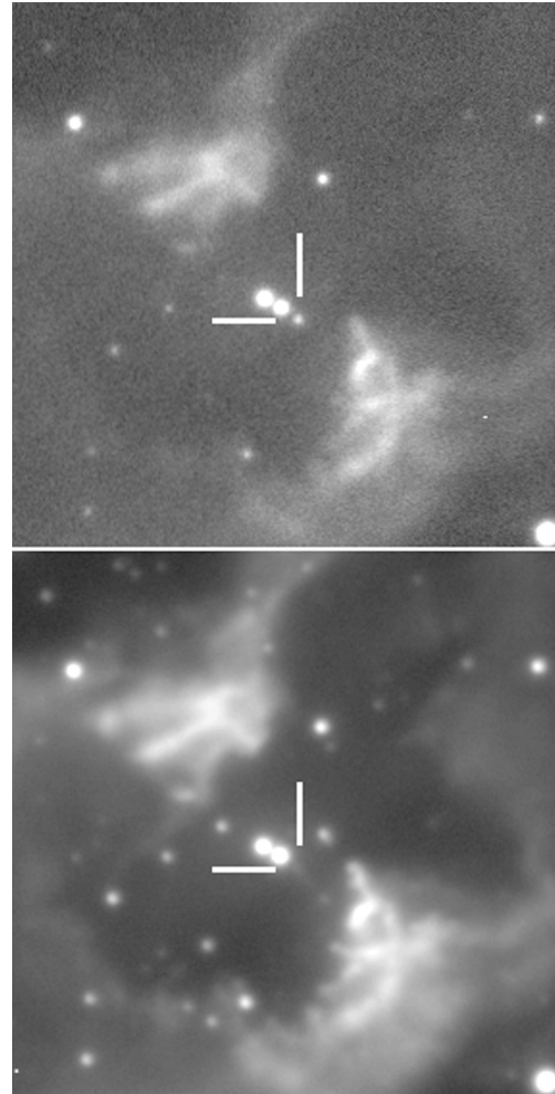
Figure 23. The central star of NGC 2899 reveals itself. The top panel is a 1×1 arcmin 2 thumbnail of the centre of NGC 2899 as imaged through the u filter, while the bottom is the corresponding r thumbnail. The white right-angled bars pick out the position of an extremely blue, relatively faint star that is clearly present in all u (and g ) exposures obtained, but is too faint for detection in r .
