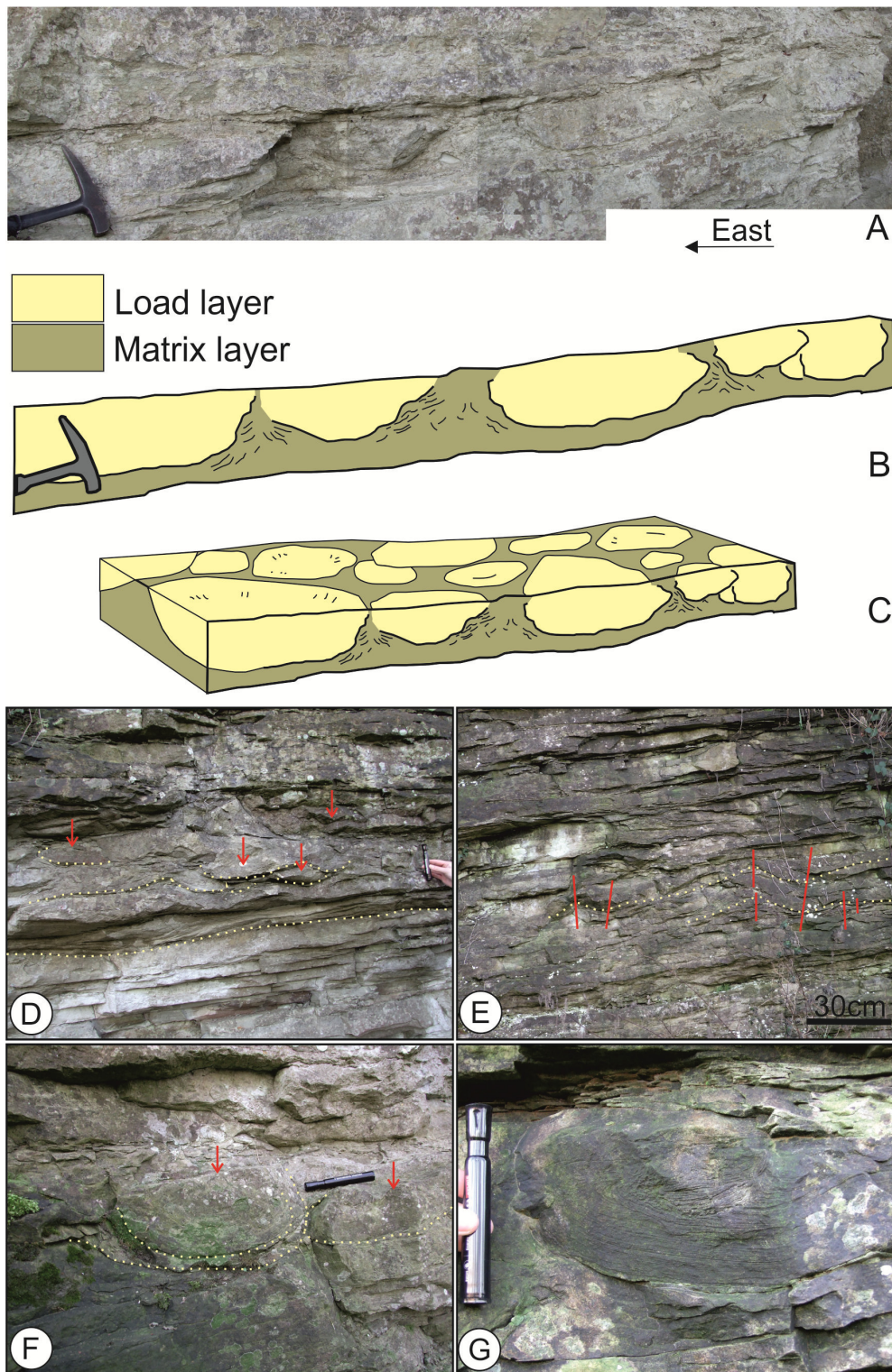
Figure 6. Examples of load casting and convolute bedding exposed in the old Whitcliffe quarry. (A) Photo montage of a well exposed section of the lower deformation horizon towards the top of the Lower Whitcliffe Formation, 2.4 m below the contact with the Upper Whitcliffe Fm. Undeformed strata can be observed both above and below the soft sedimentary deformation. Several prominent load casts with associated dewatering features are shown. Hammer head for scale (17 cm). (B) Schematic interpretation of A, the relationship between the load and matrix layers is highlighted. (C) Three dimensional interpretation of the load casts as thixotropic bowls. (D) Further examples of the load casts (arrows) with several convolute bedding planes highlighted (dashed lines). (E) Photograph showing several prominent convolute beds, highlighted as dashed lines; axial traces have been included displaying the vertical/very steep nature of the convulsions; no vergence is apparent. (F) Photograph showing the relationship between adjacent load casts (arrows); matrix material is often seen to be injected between the loads to create dewatering structures. Such structures are referred to as flame structures. (G) Photograph of an individual load cast. At this scale internal deformation can be observed within the larger structure. The small scale soft sedimentary deformation includes convolute laminae and small scale dewatering features. Pen for scale in D, F and G (14 cm).
