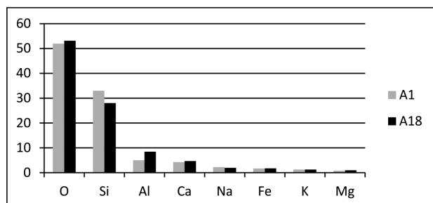
Figure 5. Bar chart summarising multi point analysis results. Y axis = weight percentage. A1 and A18 have very similar compositions, indicating that there is no compositional difference throughout the Whitcliffe Formations at the old Whitcliffe quarry.
