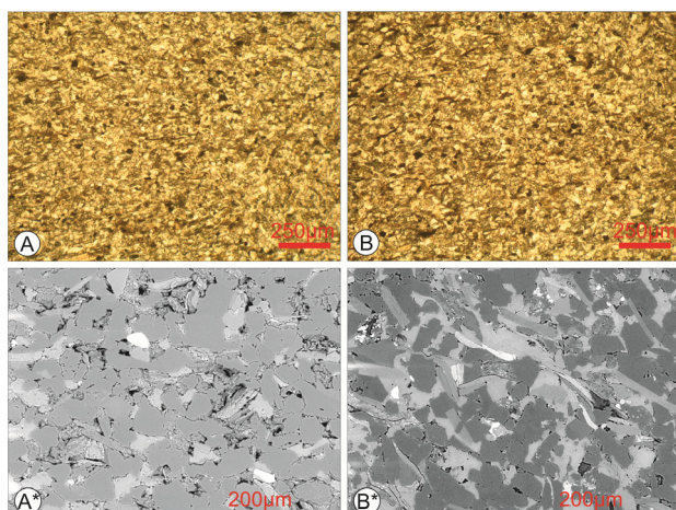
Figure 4. A and B are photomicrographs from slides of A1 and A18 respectively. A* and B* are Back Scatter Electron images of samples A1 and A18 respectively. Compositionally the samples are the same, grains are slightly smaller in A18 than A1. Note: colour difference in A* and B* is due to a difference in contrast whilst imaging.
