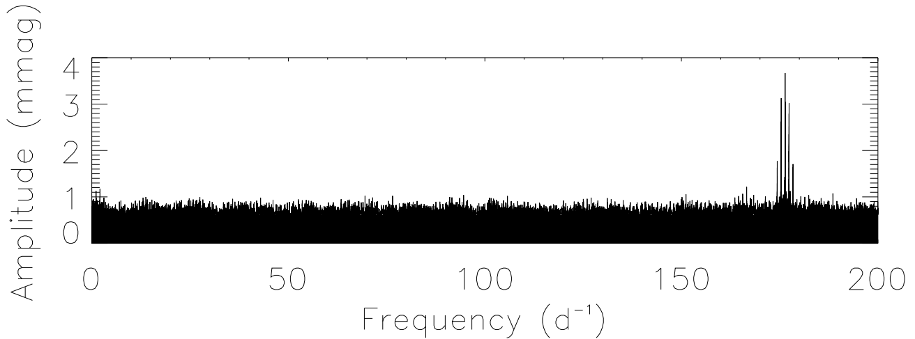
Figure 5. Periodogram of all seasons of WASP data. The data have been pre-whitened to 10\text{ d}^{-1} to the approximate noise level of the high-frequency range to remove the rotation signature and low-frequency noise. Note that the structure surrounding the pulsation signature is a result of daily aliases.
