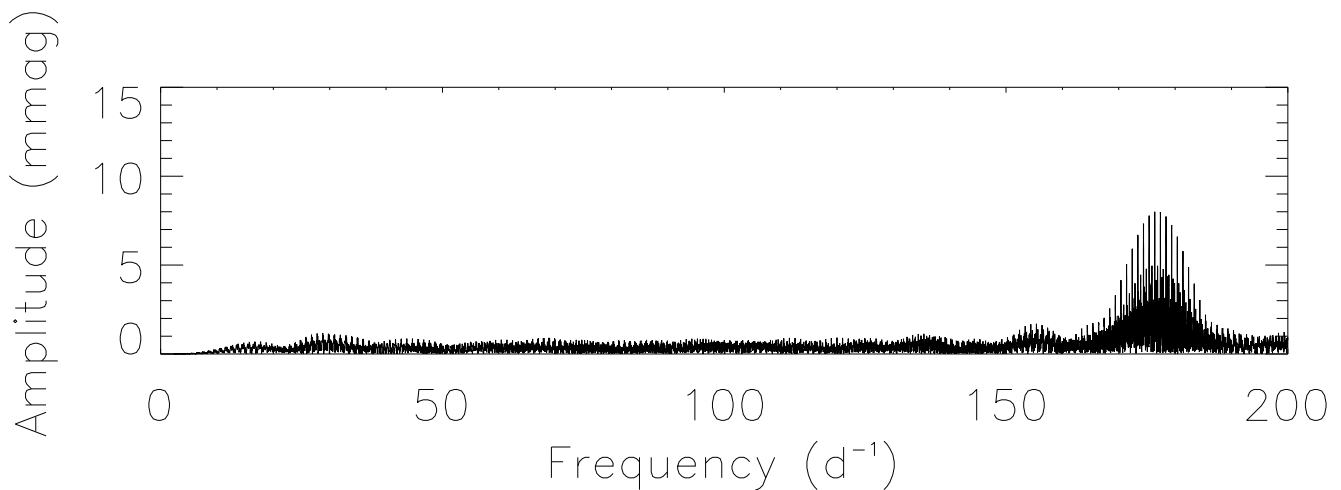
Figure 7. Periodogram of the 2014 SAAO data set. The pulsation is clearly present at 176.39 \text{ d}^{-1} with an amplitude of 8.00 mmag. The structure surrounding the peak are daily aliases.
