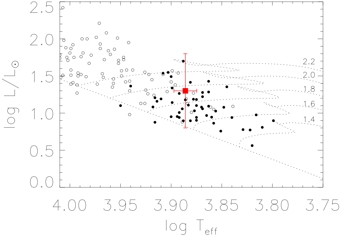
Figure 1. The positions of the roAp stars for which GAIA or Hipparcos parallaxes are available (filled circles). We include the non-oscillating Ap stars for comparison (open circles) for which there is reliable data, and non-detections, in the literature. The subject of this study, J1940, is shown by the red square, with its position determined in sections 2 and 4. The zero-age main-sequence and the evolutionary tracks are from Bertelli et al. (2008). Note, we do not plot the error bars of the other stars for clarity; these are typically \pm 0.02 and \pm 0.3 in \log T_{\text{eff}} and \log L/L_{\odot} , respectively.
