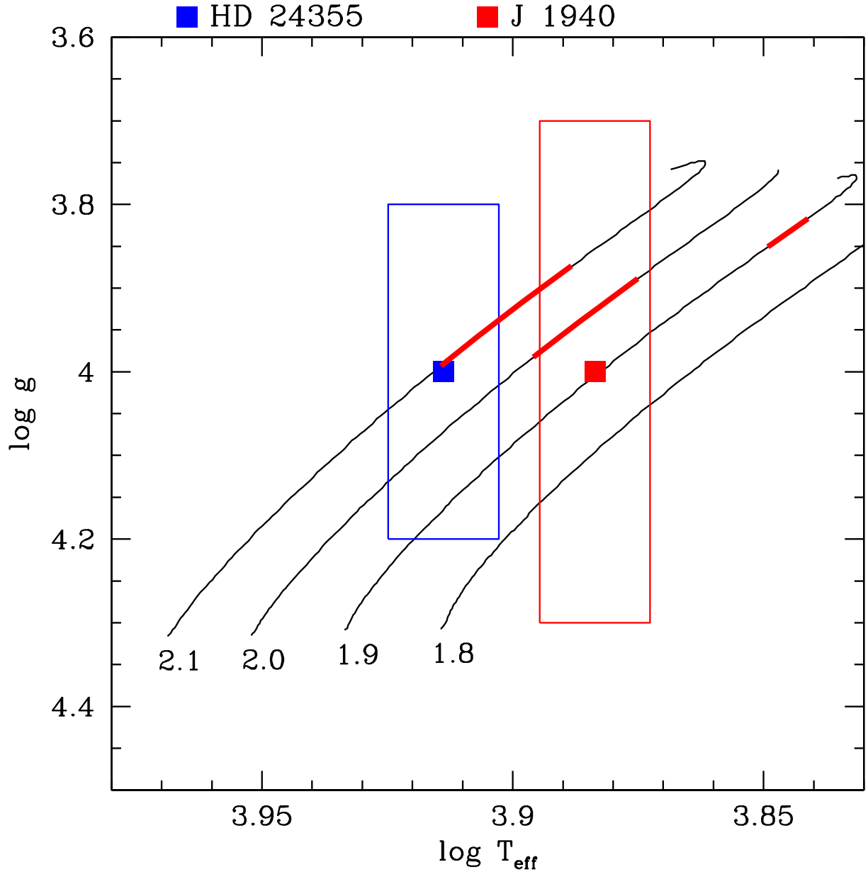
Figure 16. The \log T_{\text{eff}} - \log g diagram showing the approximate positions of J1940 and HD24355 with error boxes, and evolutionary tracks of 1.8, 1.9, 2.0, and 2.1 M_{\odot} stars. The thick red lines along the evolutionary tracks indicate the positions where theoretical amplitude/phase modulation curves reproduce satisfactorily the observed ones of J1940.
