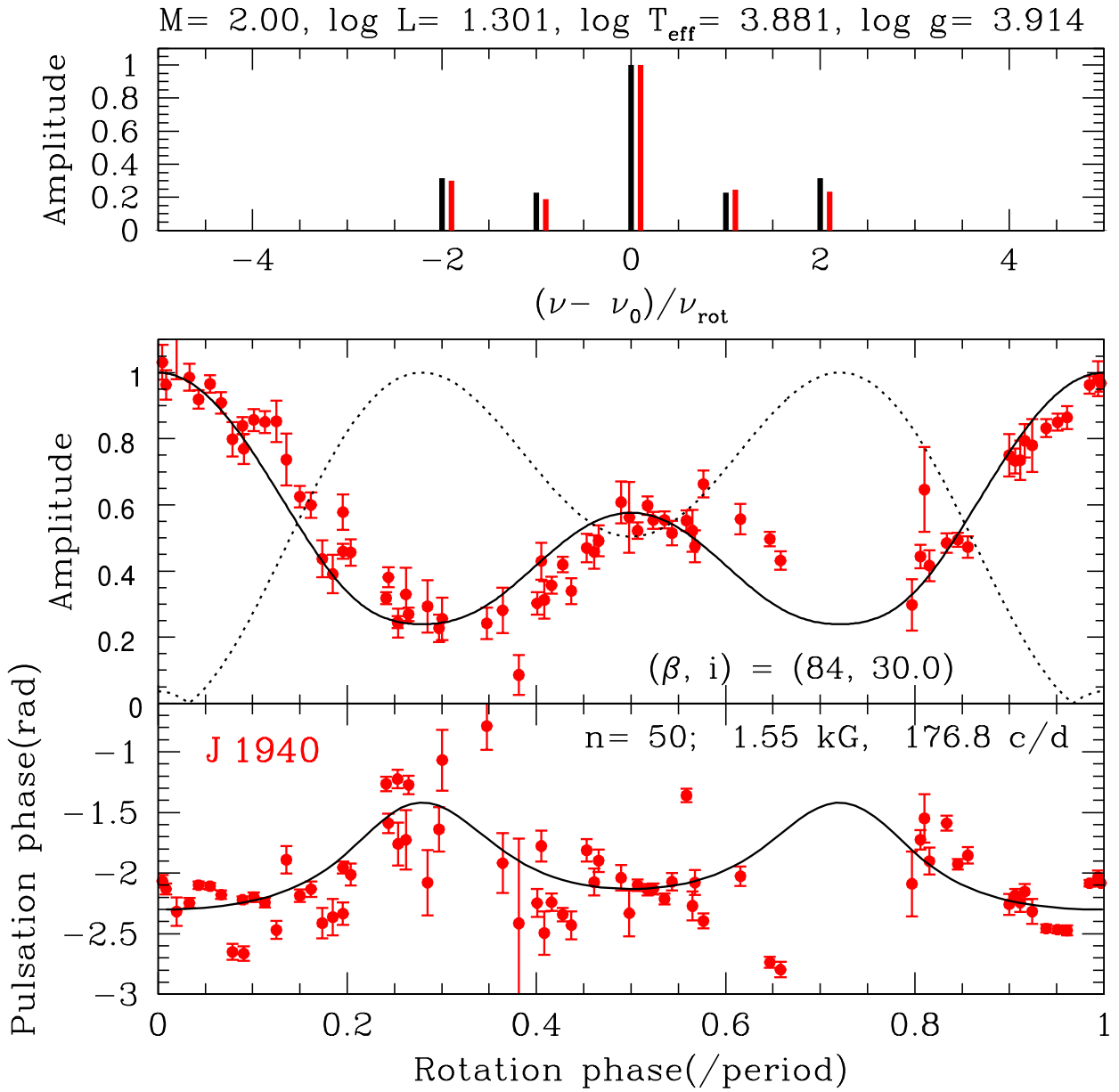
Figure 15. Comparison of amplitude and phase modulations between a model and observational results of J1940. Red and black colours are used for J1940 and the model results, respectively. Top: comparison of the rotational sidelobes, in which the observations are slightly shifted rightward for visibility. Middle: comparison of the amplitude modulations as a function of the rotation phase. The solid line is a theoretical amplitude modulation computed by taking into account the magnetic effects, while the dotted line indicates the amplitude modulation expected from a pure quadrupole. Bottom: comparison of the modulations of the pulsation phase as a function of the rotation phase; the black line represents the model result, while the red dots with error bars are observational results for J1940.
