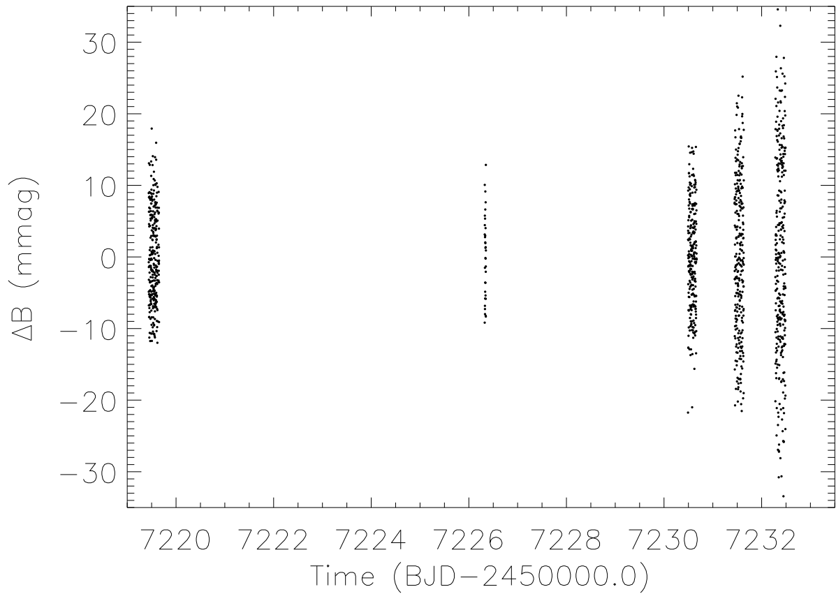
Figure 8. Light curve of the 2015 data from the SAAO, where the data have been binned to 60 s integrations. Clearly evident is the night-to-night pulsational amplitude variation.
