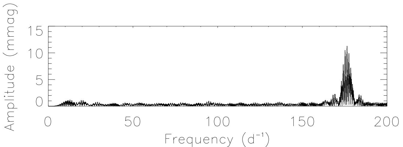
Figure 9. Periodogram of the 2015 SAAO data set. The pulsation is clearly present at 176.39 \text{ d}^{-1} with an amplitude of 11.29 mmag.
