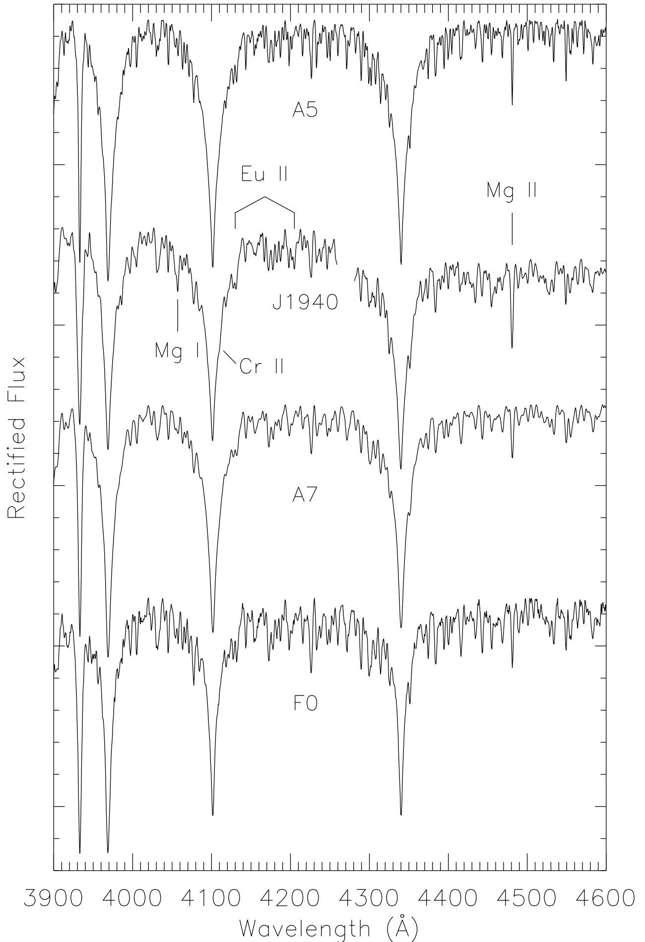
Figure 2. Spectrum of J1940 (second) compared to MK standard stars of A5 type (top), A7 type (third) and F0 type (bottom). The target spectrum has been convolved with a Gaussian profile to the resolution of the MK standards (1.67 Å). The spectra have been offset for clarity.
