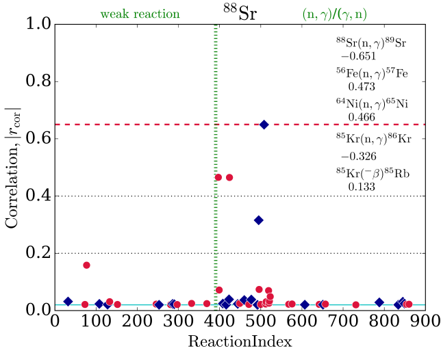
Figure 14. The correlation coefficients of reactions with respect to an abundance change of ^{88}\text{Sr} during the ^{13}\text{C} -pocket conditions. The absolute values of the coefficients are plotted against a reaction index number. Red circles stand for positive correlation and blue squares for negative correlation, respectively. Reaction indices in the range of 1–390 denote weak reactions and those in the range 391–900 identify neutron captures. The five reactions with the highest correlations are listed in the upper right corner. Note that, for better readability, reactions with correlation factors |r_{\text{cor}}| < 0.02 are omitted from this plot.
