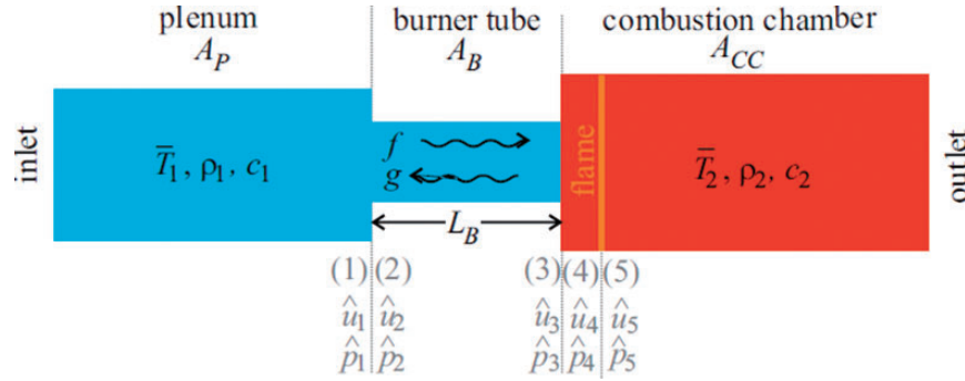
Figure 26. Schematic of a combustion system comprising three cavities: plenum (cold), burner tube (cold), and combustion chamber (hot). Points (4) and (5) are infinitesimally close; they are drawn with a distance between them to visually separate the flame from the jump in cross-section.
