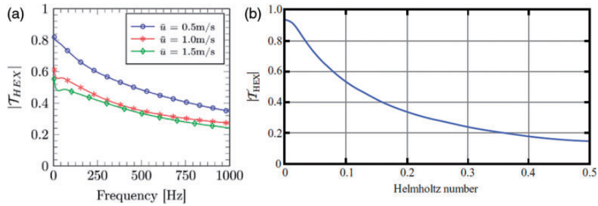
Figure 46. Numerical results for the gain of the HEX transfer function. (a) Results for the circular geometry in Figure 45(a) with d = 3 \text{ mm} and h_g = 0.3 \text{ mm} (from Figure 4(a) in Surendran et al. 90 ) and (b) Results for the rectangular geometry in Figure 45(b) with d = 12.8 \text{ mm} and h_g = 0.8 \text{ mm} (after Figure 3(a) in Strobio Chen et al. 91 ).
