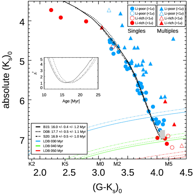
Figure 4. M_{K_s} vs (G - K_s)_0 for high probability cluster members. Red and blue symbols denote targets classed as Li-rich and Li-poor (in §4.1), where open and closed symbols denote whether the EW(Li) is within, or not within, one error bar of 300 \text{ m\AA} . Circles and triangles represent the likely-single and likely-multiple stars (in §5), respectively. The grey box denotes the estimated position of the lithium depletion boundary (LDB). The blue, green and red lines represent curves of constant luminosity at 99 per cent Li depletion from three standard models (see §4.2 for details) at 30, 40 and 50 Myr, respectively. The black curves are the best-fitting M_{K_s} vs (G - K_s)_0 isochrones to the likely single stars for the same models. The inset plot shows the reduced \chi_r^2 as a function of isochrone age.
