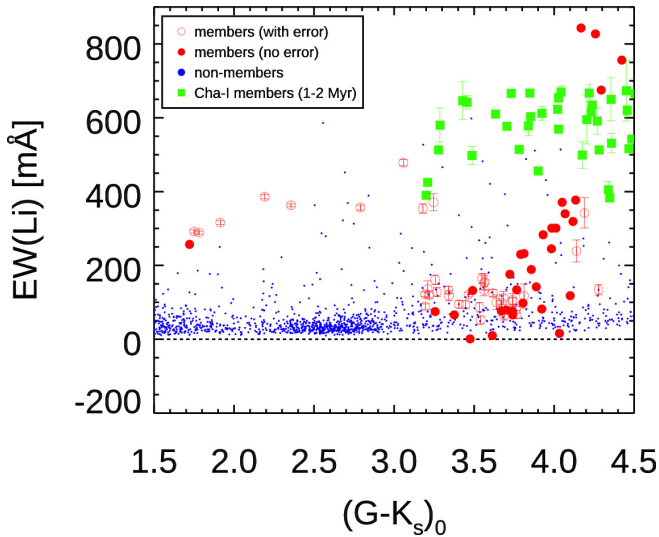
Figure 1. EW(\text{Li}) versus (G - K_s)_0 in NGC 2232, using EW(\text{Li}) measurements from GESiDR5. Red symbols represent the 80 high probability members ( P_{3D} > 0.95 ). Open and filled symbols denote EW(\text{Li}) values with and without reported uncertainties in GESiDR5, respectively. Blue points are likely non -members of NGC 2232 ( P_{3D} < 0.1 ) observed in the same instrument configurations as the members. The green squares are members of the \sim 2 Myr Cha I association also observed as part of GES.
