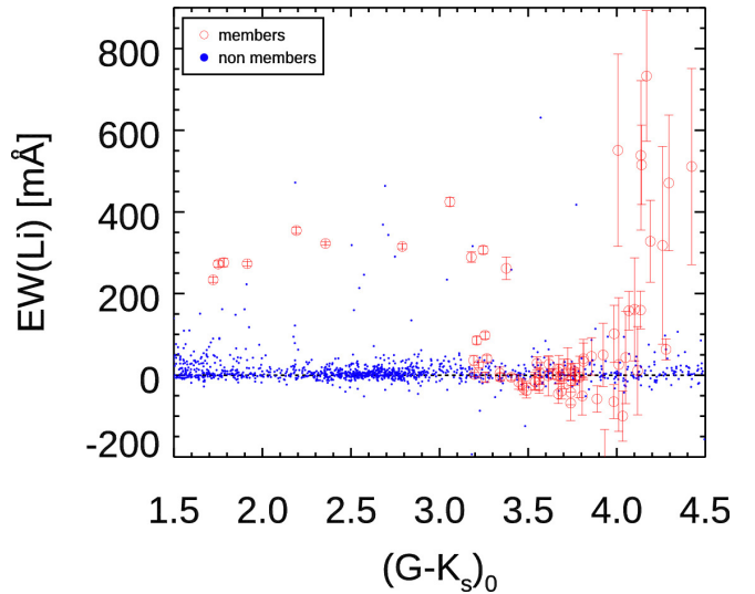
Figure 2. EW(\text{Li}) versus (G - K_s)_0 , using the revised EW(\text{Li}) values (and errors) calculated from our analysis in §3.2. The symbols and notation are the same as those described in Figure 1.
