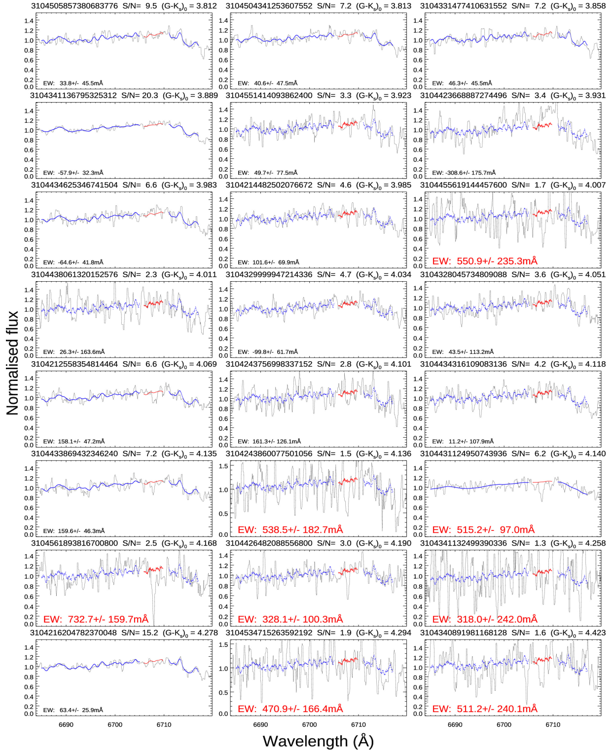
Figure 3. GES spectra for the 24 targets with (G - K_s)_0 > 3.8 . The normalised, reduced spectra from GESiDR5 are displayed in grey, where the data have been binned by 7 pixels. The best-matching spectral template (described in §3.2) is shown in the region encompassing the Li-feature at 6708 Å (in red) and in two regions either side of the feature (in blue). The title of each panel gives the Gaia DR2 source identifier, the SNR given in GESiDR5 and the (G - K_s)_0 colour. The EW(Li) values are provided in the bottom-left of each panel, where targets defined as Li-rich are highlighted in larger red text.
