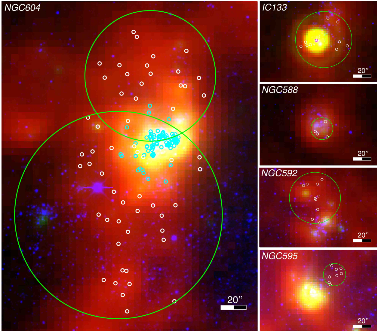
Figure 17. RGB image ( 250\mu\text{m} Herschel -SPIRE, 24\mu\text{m} Spitzer -MIPS, \text{H}\alpha respectively – see Sect. 2.2 for image details) of NGC 604, IC 133, NGC 588, NGC 592 and NGC 595. YSOs identified in this work are shown by white circles, the extent of each SFR is shown by the green circles, in NGC 604 cyan circles show YSOs identified in Fariña et al. (2012) , in IC 133 the magenta circle shows the location of the maser counterpart (see text).
