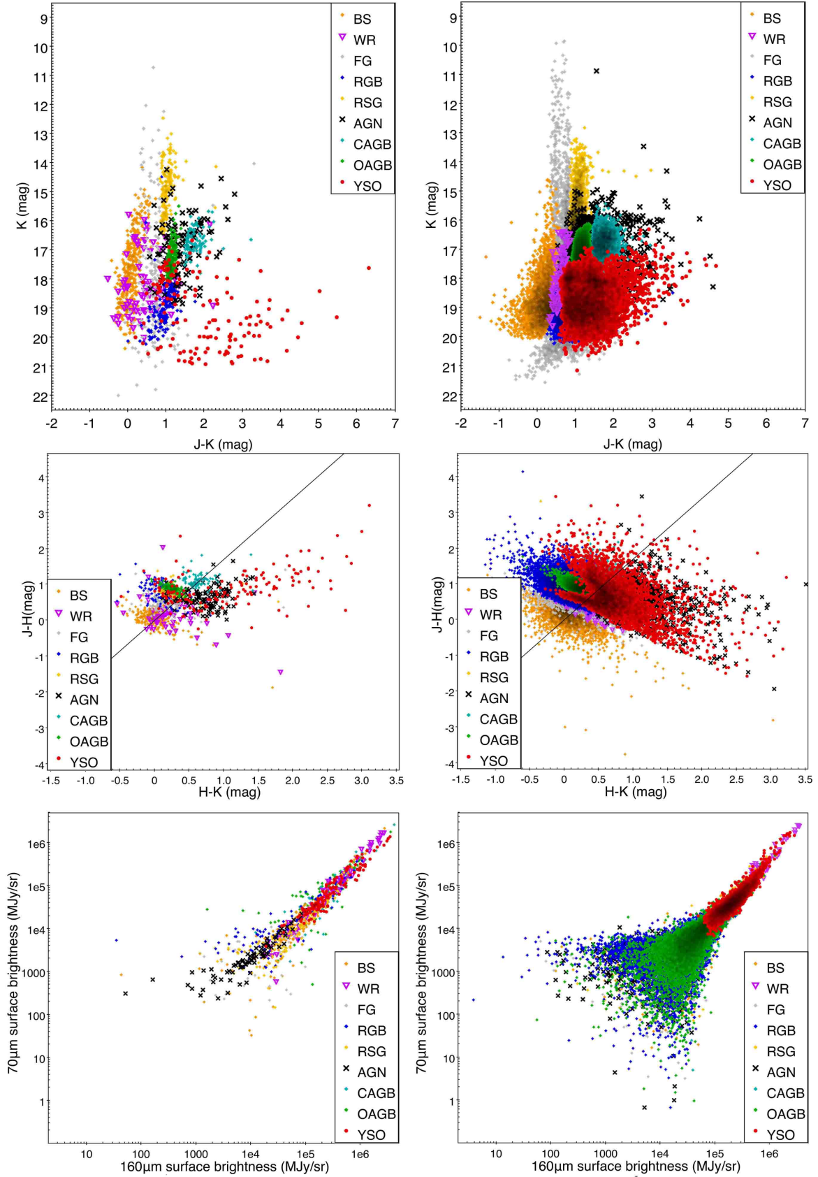
Figure 7. CMD, CCD and far-IR brightness plots of the training set sources (left) and for the classified sources (right). Colour-coding is given in the legend. The reddening line shown in the CCD plots is derived using the coefficients from Rieke & Lebofsky (1985) .
