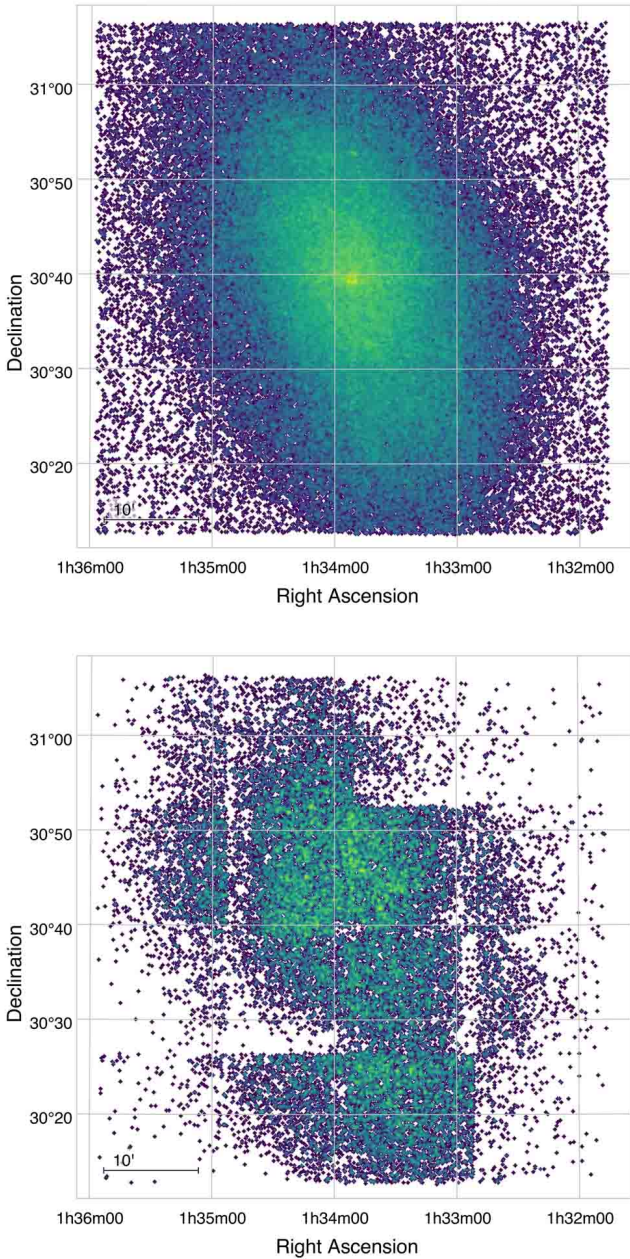
Figure 2. Hess diagrams of source density, brighter (top) and fainter (bottom) than K_s = 19.2 mag. The effect of variable depth in the catalogue across the field-of-view is clear at fainter magnitudes.
