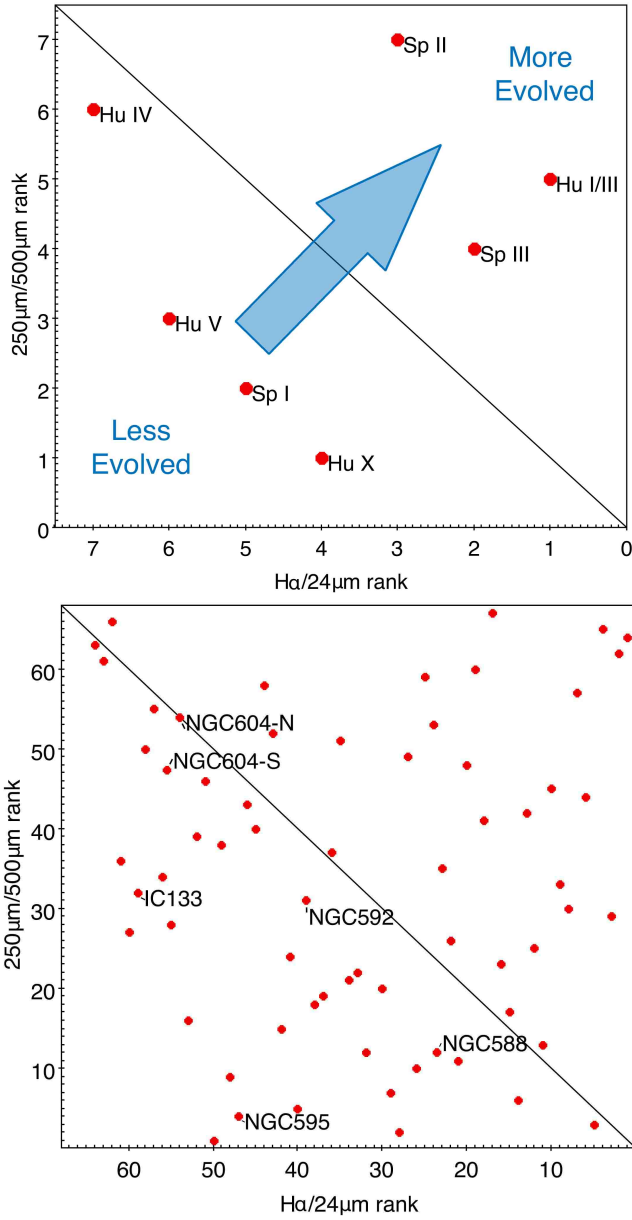
Figure 13. SFRs in NGC 6822 (upper) and M 33 (lower) shown by their relative ranks in the [H\alpha]/[24\mu m] and [250\mu m]/[500\mu m] ratios. The diagonal line indicates the locus of equal rank in both ratios. In the top panel the direction of SFR evolution is indicated by the arrow; significant SFRs are labelled (see text for more detail).
