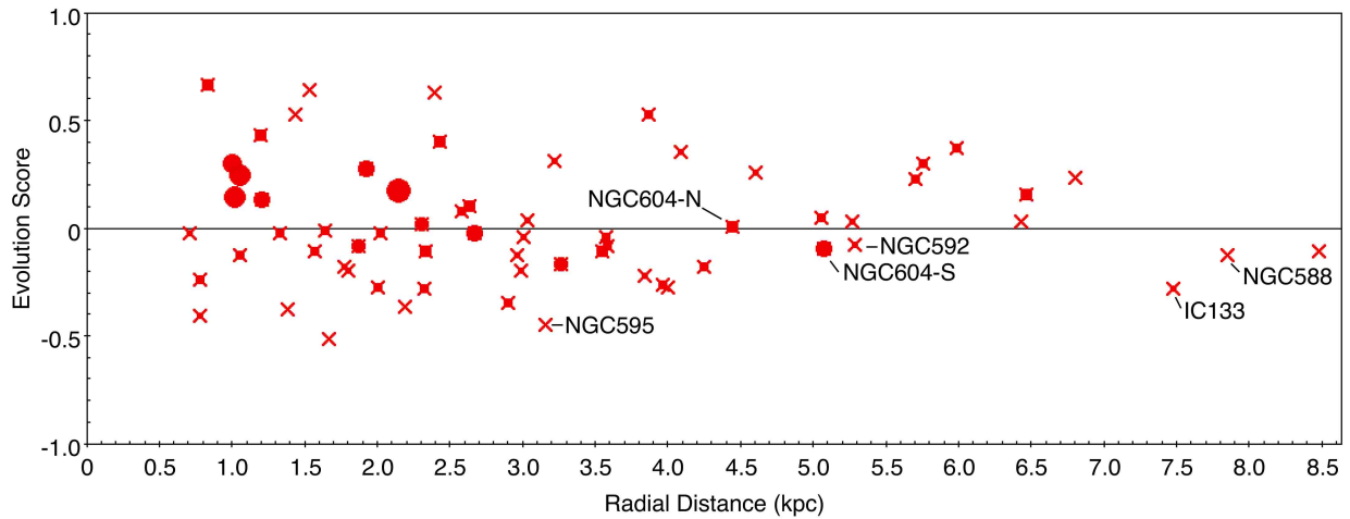
Figure 15. Normalised evolution score against radial distance for SFRs in M33. Symbol size is proportional to the radius of each cluster. IC 133 and NGC 588 are notable outliers in that they have a low evolution score and lie far out in the disk of M33.
