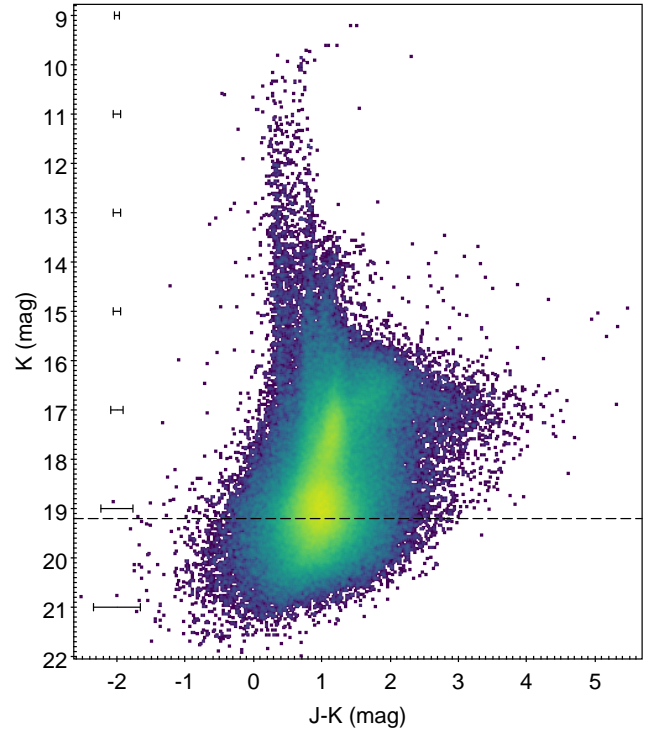
Figure 3. The near-IR catalogue presented in a CMD Hess diagram. Average error bars are shown. The dashed line at K_s = 19.2 mag indicates the magnitude at which the catalogue depth becomes very patchy (Fig. 2).
