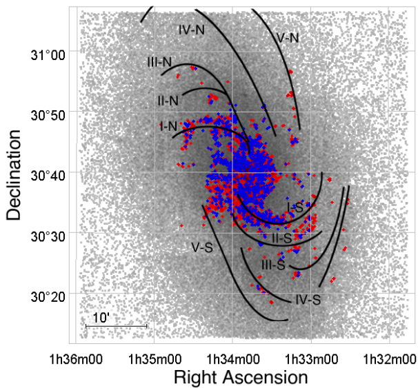
Figure 9. YSO distribution in M33, with the spiral structure adapted from Humphreys & Sandage (1980) overlaid (colour-coding as in Fig. 8).
