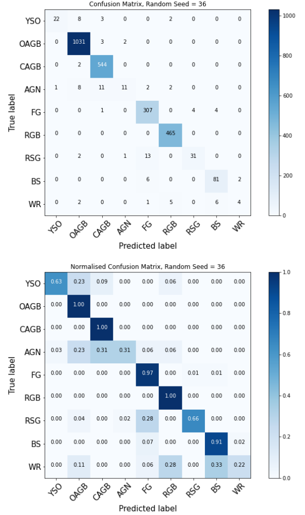
Figure 5. Non-normalised (top) and normalised (bottom) confusion matrices for an example PRF run with no class down-sampling (see text). The large classes achieve high accuracy, however for the smaller classes high levels of confusion are evident.
