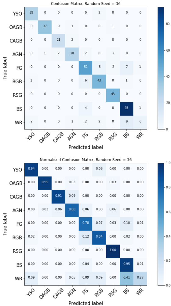
Figure 6. Non-normalised and normalised confusion matrices (respectively top and bottom) for the PRF run using the same random seed as those shown in Fig. 5, but here with class down-sampling (see text). The misclassifications for the smaller classes are very effectively reduced.
