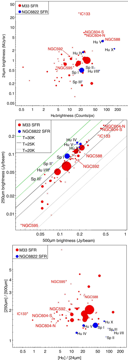
Figure 12. Photometric measurements for each SFR in M33 and NGC 6822 (red and blue symbols respectively): H\alpha and 24\mu\text{m} (upper panel), 250 and 500\mu\text{m} (middle), [H\alpha]/[24\mu\text{m}] and [250\mu\text{m}]/[500\mu\text{m}] (lower). The symbol size is proportional to the number of YSOs in each region (crosses mark particularly small regions); SFR radii for M33 and NGC 6822 are respectively from our analysis and from Kinson et al. (2021) . In the middle panel loci for modified blackbodies of different temperatures (colour-coded) and \beta = 2 and 1.5 (solid and dashed lines respectively) are shown. Significant SFRs are labelled (see text).
