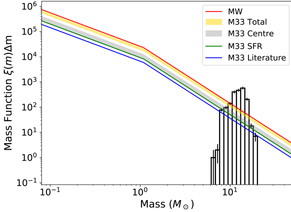
Figure 18. The mass distribution of the 1986 YSOs assigned to M33 SFRs, with scaled Kroupa (2002) IMFs overlain, see text for details. Poisson errors are indicated for each histogram bin.
