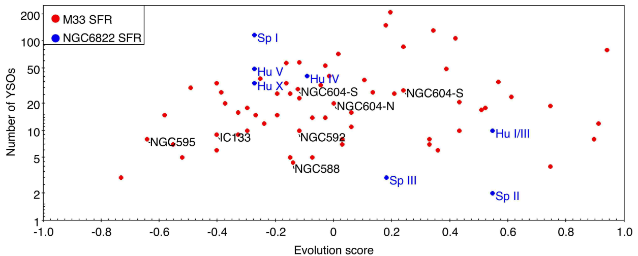
Figure 16. Number of YSOs against normalised evolution scores for SFRs in M33 and NGC 6822. The number of YSOs for SFRs in M33 and NGC 6822 are respectively from our analysis and from Kinson et al. (2021) . There seems to be a slight tendency for larger SFRs to appear more evolved in M33.
