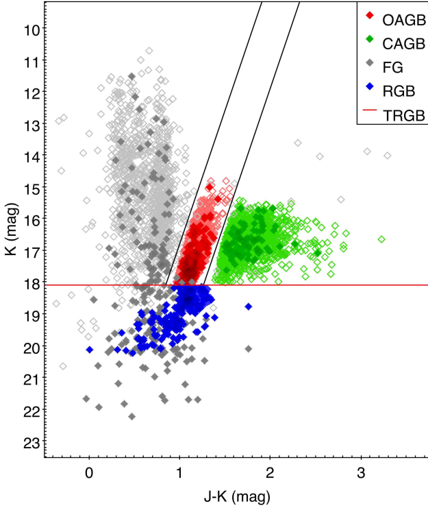
Figure 4. A CMD showing the four large classes which were down-sampled with the full set of data shown by open symbols and the down-sampled data by filled symbols. The parameter space for each class is well represented by the down-sampled data. The TRGB magnitude ( K_s = 18.11 mag) and AGB colour-cuts adapted from Ren et al. (2021) are shown by the red and black lines respectively.
