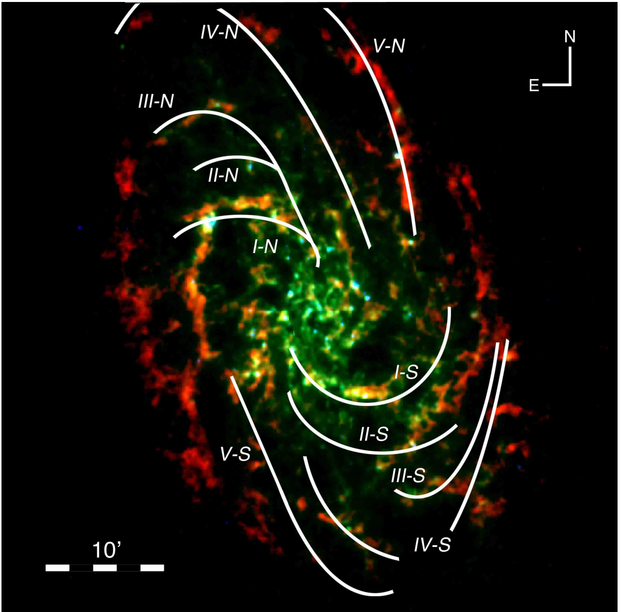
Figure 1. An RGB image of M 33, showing VLA H I (red, Gratier et al. 2010), 250 \mu\text{m} Herschel -SPIRE (green, Kramer et al. 2010), 24 \mu\text{m} Spitzer -MIPS (blue, Engelbracht et al. 2004). The figure covers the same footprint as the near-IR WFCAM catalogue of Javadi et al. (2015). The spiral arm identifications, adapted from Humphreys & Sandage (1980), are shown in white.
