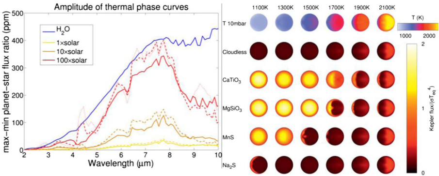
Fig. 14 Left: Figure from Charnay et al. [48]. Amplitude of thermal phase curves of a warm sub-Neptune similar to GJ1214b without cloud (solid lines) and with cloud (dashed lines for radii of 0.5 μm and dotted line for radii of 0.1 μm) for metallicity of 1, 10, 100 and a pure water atmosphere. Right: Figure from Parmentier et al. [172]. Temperature and outgoing flux from the dayside of hot Jupiters with different equilibrium temperatures. The first row shows the temperature at 10 mbar estimated by a global circulation model. The following rows show the total flux (emitted + reflected) from the dayside hemisphere in the spectral range observed by the Kepler spacecraft. The second row is a model without clouds, whereas in the subsequent rows one cloud species is condensing
