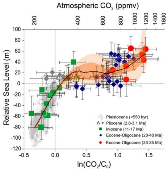
Figure 16. Sea level versus CO 2 concentrations (and the logarithmic radiative forcing influence of CO 2 changes expressed by \ln(CO_2/C_0) , where C 0 represents the preindustrial CO 2 level of 278 ppmv) (after Foster & Rohling, 2013). Symbols represent reconstructions with uncertainties for different intervals of the past 40 million years. The black line and orange envelopes represent a probabilistic assessment that takes into account full propagation of all uncertainties (black line is the probability maximum; dark orange is the 68% probability interval; light orange is the 95% probability interval).
