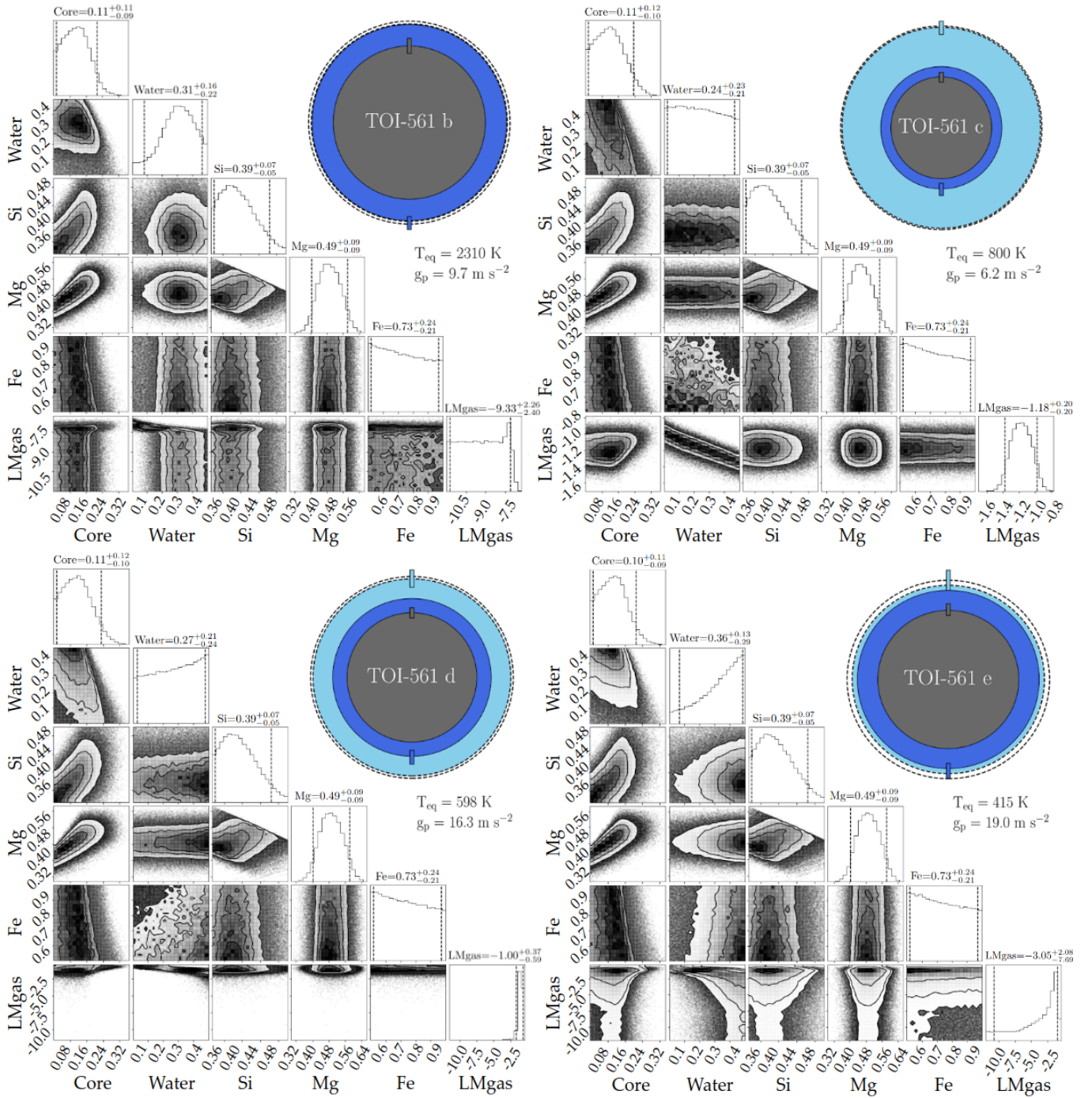
Figure 13. Posterior distributions of the main parameters describing the internal structure of TOI-561 b ( top left ), c ( top right ), d ( bottom left ), and e ( bottom right ). Each corner plot shows the mass fraction of the inner core and of the water layer, the molar fractions of silicon and magnesium in the mantle, the iron molar fraction in the inner core, and the mass of gas in logarithmic scale. On top of each column are printed the mean and the 5 per cent and 95 per cent quantiles values. For each planet, and we show an illustration of the radius fractions of the inner core+mantle (dark gray), water layer (dark blue), and gas envelope (light blue), corresponding to the medians of the posterior distributions. The coloured rectangles indicate the uncertainty on the corresponding layer thickness, while the black dashed outer rings represent the uncertainty on the total radius. Equilibrium temperature and planetary surface gravity are reported for each planet.
