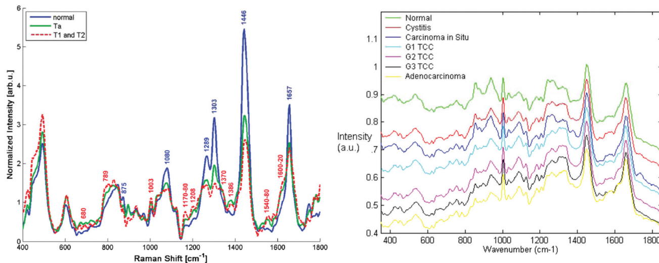
Fig. 3 Comparison of Raman spectra from the bladder surface (left) measured using a six collection fibres around one illumination fibre probe with no beam steering/focussing at 785 nm (ref. 101 reproduced with permission) and (right) Raman spectra measured from bladder biopsy surface using a semi-confocal, 830 nm Raman microspectrometer (ref. 102 reproduced with permission). The right hand spectra are the 'true' surface spectra, most demonstrating early malignant changes, whereas the in vivo spectra show spectra combining the spectral signals from all layers in the bladder wall including the adipose tissue surrounding the outside of the bladder wall. This is clear from the highly lipid-rich spectra and highlights the importance of designing probes to optimally sample tissue regions/volumes of interest.
