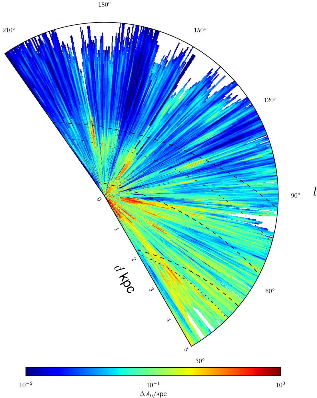
Figure 5. A map of extinction at b = 0 , after convolution with a uniform kernel to reduce the resolution to 0^{\circ}.25 in l and 500 pc in distance, so as to roughly match the resolution of fig. 9 of Marshall et al. (2006). The sun lies at the plot's origin with the Galactic Centre off the bottom of the plot. The dashed lines denote the position of the Sagittarius, local and Perseus spiral arms given by Reid et al. (2014), whilst the dot-dashed lines correspond to the Sagittarius and Perseus arms of Vallée (2013). Note the non-physical ‘fingers of God’ – discontinuities in the azimuthal direction.
