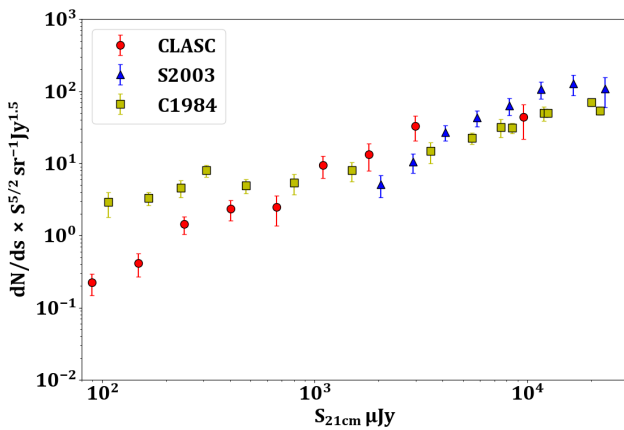
Fig. 8. Normalised differential source counts. CLASC sources are represented by red circles and are compared against the source counts from other surveys at 21 cm by Setia Gunawan et al. (2003, blue triangles) and Condon & Mitchell (1984, yellow squares).
