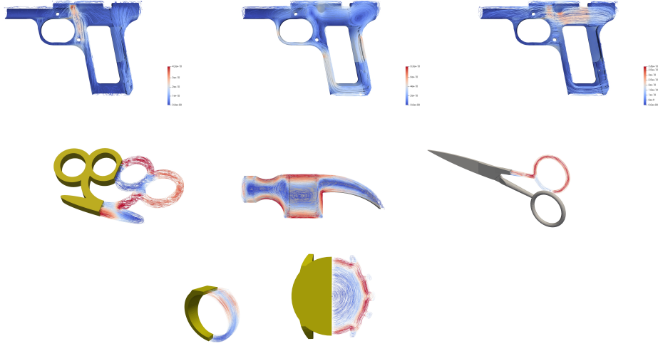
Figure 12: Set of multiple threat and non-threat objects: Illustrative contours of \mathbf{J}_i^e = i\omega\sigma_*\theta_i at \omega = 1 \times 10^4 rad/s for a sample of the threat and non-threat objects.
