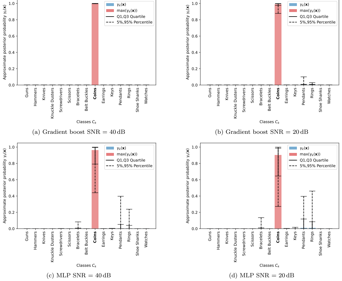
Figure 19: Set of multiple threat and non-threat objects: Approximations p(C_k|\mathbf{x}) \approx \gamma_k(\mathbf{x}) to posterior probabilities p(C_k|\mathbf{x}) , k = 1, \dots, K , where (\mathbf{x}, \mathbf{t}) \in D_{15}^{(\text{test}, (9))} (Coins) for P^{(k)} = 5000 when K = 15 showing (a) gradient boost SNR = 40 dB, (b) gradient boost SNR = 20 dB, (c) MLP SNR = 40 dB and (d) MLP SNR = 20 dB.
