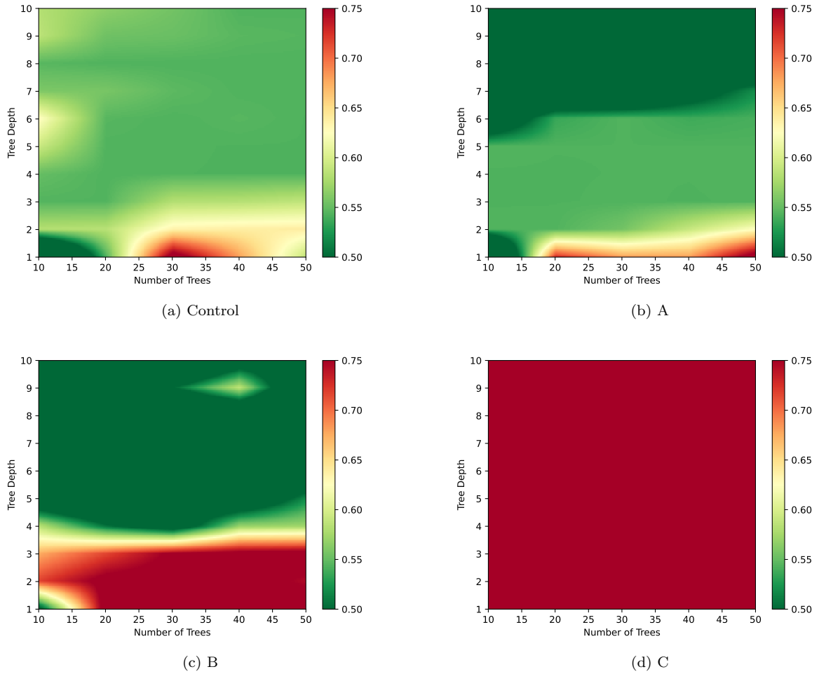
Figure 22: Set of multiple threat and non-threat objects: Overall performance of the gradient boost classifier for different values in the hyperparameter space, with P^{(k)} = 2000 with K = 8 and \text{SNR} = 40 dB, showing average \kappa score for different values n_estimators and max_depth , for different scaling regimes (a) Control, (b) A, (c) B and (d) C.
