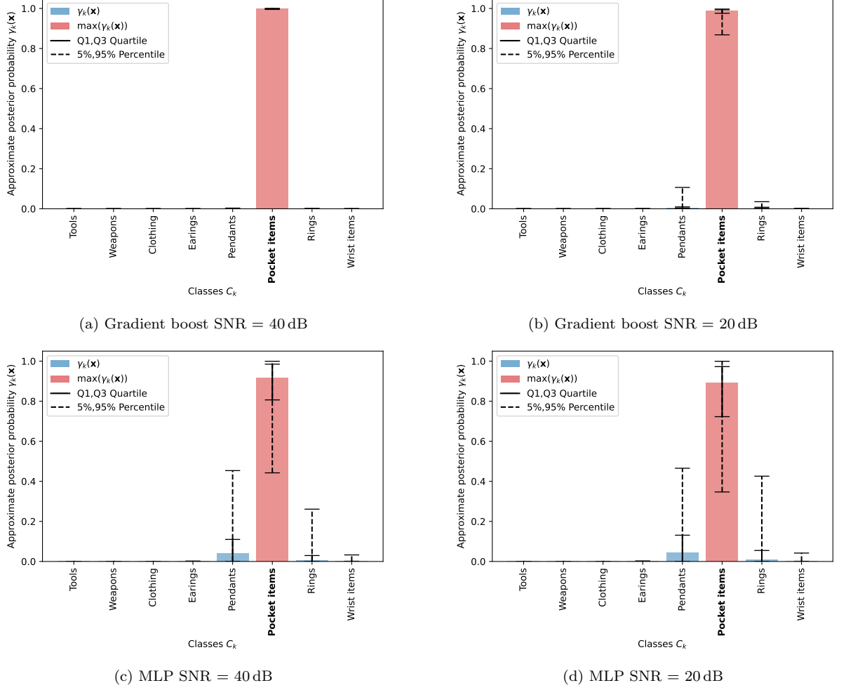
Figure 16: Set of multiple threat and non-threat objects: Approximations p(C_k|\mathbf{x}) \approx \gamma_k(\mathbf{x}) to posterior probabilities p(C_k|\mathbf{x}) , k = 1, \dots, K , where (\mathbf{x}, \mathbf{t}) \in D_8^{(\text{test}, (2))} for P^{(k)} = 5000 when K = 8 showing the classifiers (a) gradient boost SNR = 40 dB, (b) gradient boost SNR = 20 dB, (c) MLP SNR = 40 dB and (d) MLP SNR = 20 dB.
