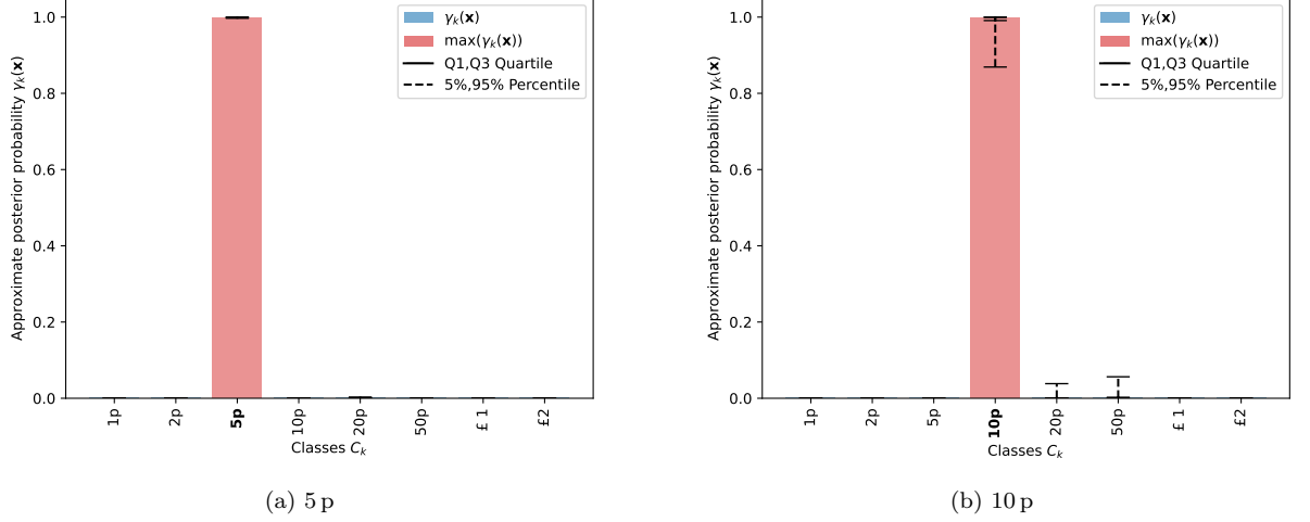
Figure 8: Set of British coins: Approximations p(C_k|\mathbf{x}) \approx \gamma_k(\mathbf{x}) to posterior probabilities p(C_k|\mathbf{x}) , k = 1, \dots, K , using the logistic regression classifier using P^{(k)} = 2000 where (a) (\mathbf{x}, \mathbf{t}) \in D^{(\text{test}, (3))} and (b) (\mathbf{x}, \mathbf{t}) \in D^{(\text{test}, (4))} .
