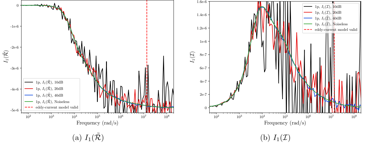
Figure 2: Set of British coins: 1 p coin \alpha B , \alpha = 0.001 m, \mu_r = 1 and \sigma = 4.03 \times 10^7 S/m showing the spectral signatures for noiseless and realisations of noise with SNRs of 40 dB, 20 dB and 10 dB (a) I_1(\tilde{\mathcal{R}}[\alpha B, \omega, \sigma_*, \mu_r]) and (b) I_1(\mathcal{I}[\alpha B, \omega, \sigma_*, \mu_r]) .
