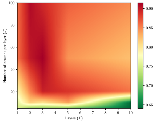
Figure 14: Set of multiple threat and non-threat objects: Overall performance of MLP for different uniform network architectures, with P^{(k)} = 5000 when K = 8 and SNR = 40 dB, showing \kappa score for different numbers of hidden layers L and numbers of neurons per layer J .
