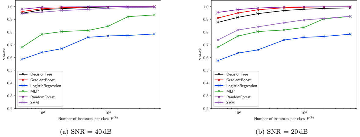
Figure 18: Set of multiple threat and non-threat objects: Overall performance of different classifiers as a function of P^{(k)} when K = 15 using the \kappa score (18) showing (a) SNR = 40 dB and (b) SNR = 20 dB.
