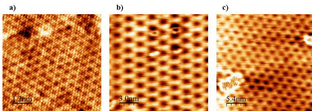
Figure V.28. STM images of SLG grown from \text{C}_{60} on: (a) Pt(111), ( 6 \times 6 \text{ nm} ), 0.11 V, 2.3 nA. (b) Ir(111), ( 15 \times 15 \text{ nm} ), 1.2 V, 2.6 pA and (c) Cu(111), ( 27 \times 27 \text{ nm} ), -0.4 \text{ V} , 2.7 pA. In every image different moiré superstructures are shown.
