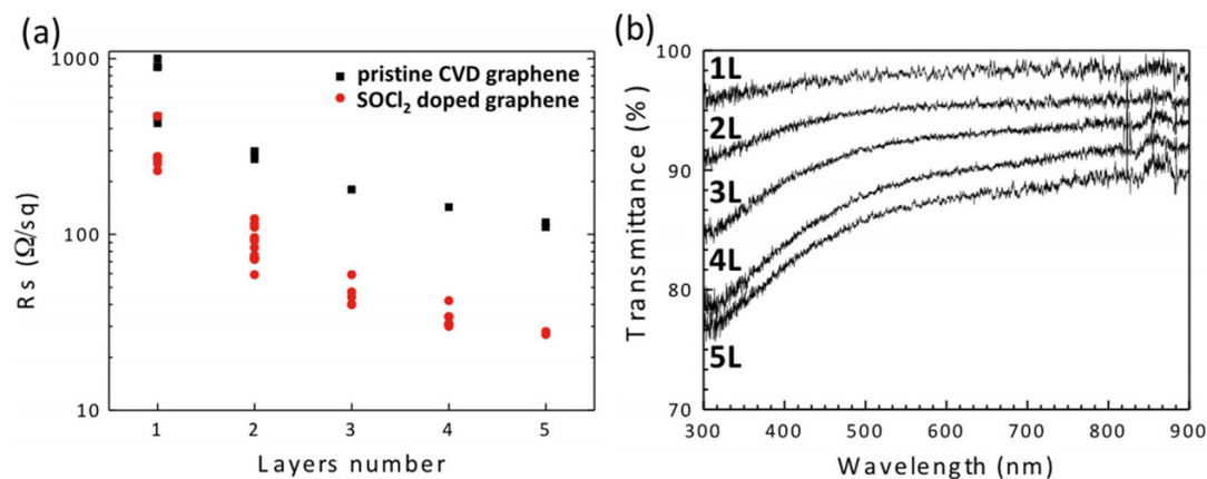
Figure VIII.5. (a) Comparison of R_s of chlorinated and non-chlorinated CVD graphene as function of N . (b) Transmittance for 1 to 5L G. Adapted from [1316].
