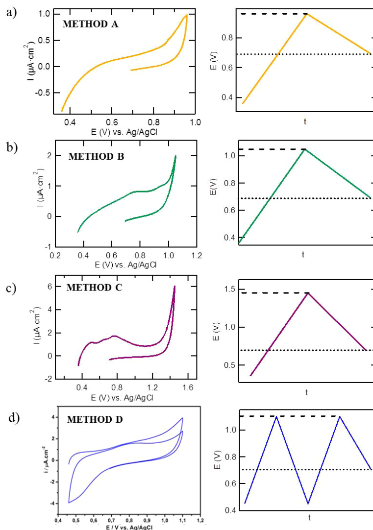
Figure VI.12. Cyclic voltammograms for graphene on Pt(111) in 0.1M aqueous HClO 4 solution. Four different voltammetric treatments have been applied (A, B, C, D), being the scan rate 0.05 V · s -1 in all the cases. The right panels plot the potential programs applied to the SLG/Pt electrodes, producing the corresponding cyclic voltammograms of the left panels.
