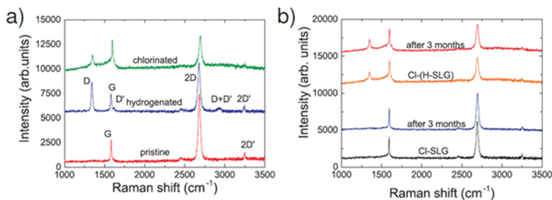
Figure VIII.6. (a) 514.5nm Raman spectra of pristine, hydrogenated and chlorinated graphene after hydrogenation. (b) 514.5nm Raman spectra of chlorinated, Cl-SLG, and hydrogenated and chlorinated graphene (Cl-(H-SLG)) directly and after doping and after three months in ambient conditions.
