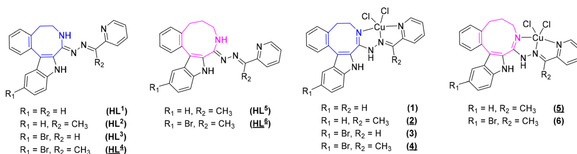
Chart 3 Indolo[2,3- e ]benzazocine and indolo[2,3- f ]benzazonine ligands and their respective copper(II) complexes synthesized in this work; underlined numbers indicate compounds studied by SC-XRD.
