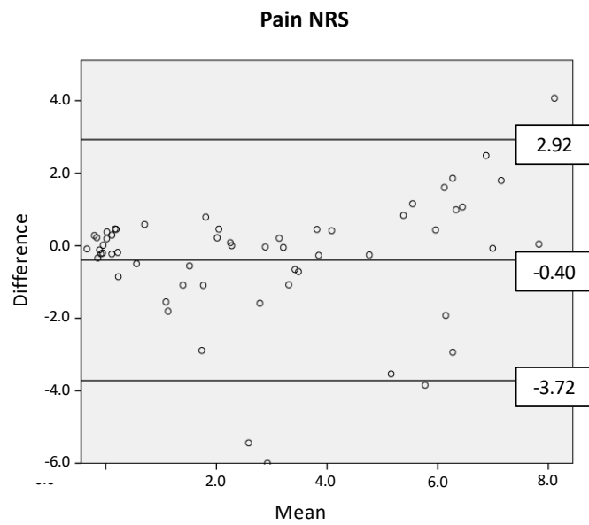
Figure 2: Bland-Altman Plots (Dataset 2)
