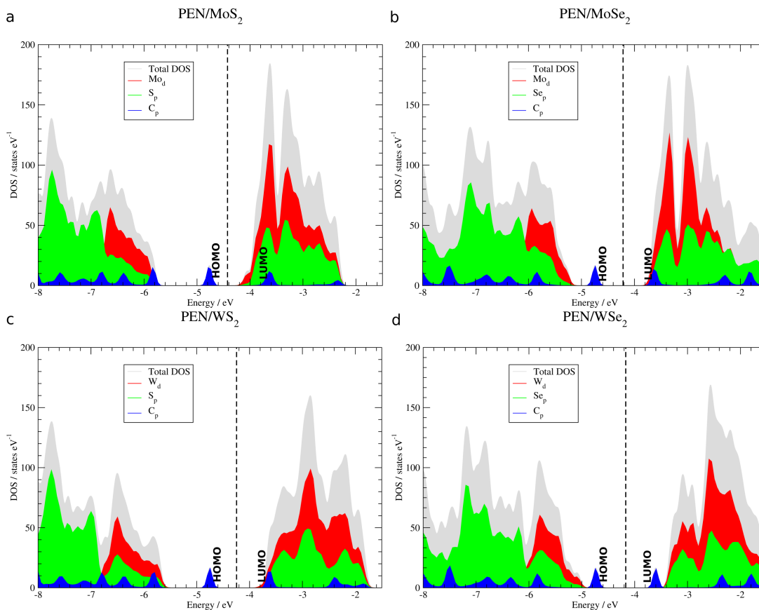
Figure 2: Total and partial density of states (DOS) of (a) PEN/MoS 2 , (b) PEN/MoSe 2 , (c) PEN/WS 2 and (d) PEN/WSe 2 heterostructures. The Fermi level of the heterostructure is indicated by a vertical dashed line. HOMO and LUMO of pentacene are highlighted in each plot.
