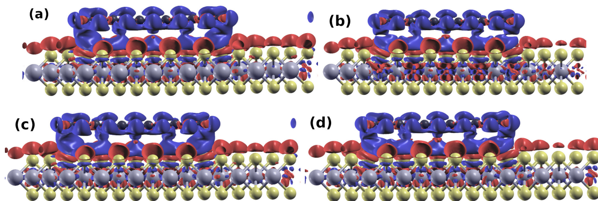
Figure 3: Charge density difference between the heterostructures ((a) PEN/MoS 2 , (b) PEN/MoSe 2 , (c) PEN/WS 2 and (d) PEN/WSe 2 ) and the isolated systems. Regions in blue and red represent depletion and accumulation of charge, respectively. Figure prepared using the XCrySDen software 45 , with isovalues in the range of -0.0001 (blue) and +0.0001 (red) e/bohr 3 .
