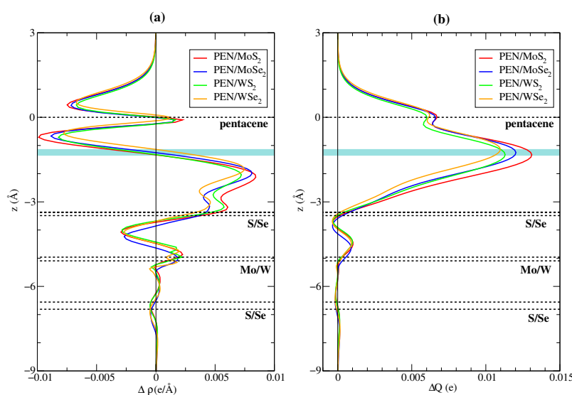
Figure 4: (a) Plane-averaged differential charge density ( \Delta\rho(z) ) calculated by integrating the charge density within the basal x - y plane at a z point. (b) Charge transferred ( \Delta Q(z) ) between pentacene and the TMDs at a z point, calculated by integrating \Delta\rho(z) from bottom to z . Horizontal dashed lines show the positions of the pentacene molecule, and the top/bottom chalcogen layers and the transition-metal layer of the TMD monolayer. Cyan region indicates the position of the interface in the PEN/TMD heterostructures.
