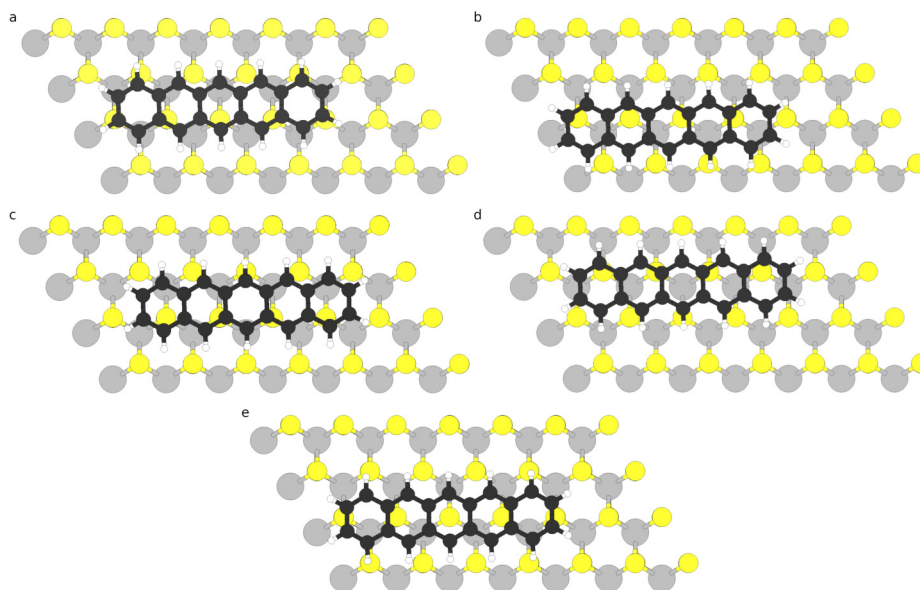
Figure 1: Ball and stick representation of the adsorption sites examined for the adsorption of pentacene molecule (horizontally oriented) on 2D monolayer TMD: (a) bridge-A, (b) bridge-B, (c) hollow, (d) top-TM, and (e) top-Ch. The adsorption sites were named based on the position of the central ring of the pentacene molecule.
