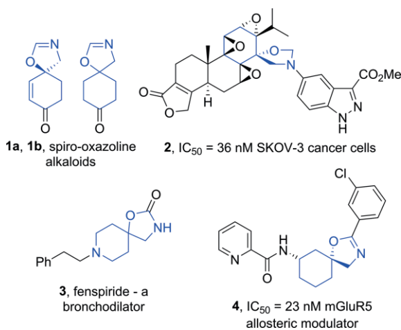
Figure 1. Examples of oxazaspirocycles.
