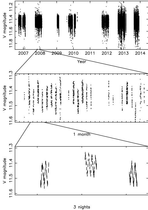
Fig. 1. Light curve of the SuperWASP data of 1SWASP J050634.16–353648.4, which contains over 56 000 data points, spanning seven years. Upper panel: complete dataset (with no error bars as they would obscure the data at this scale), illustrating the long term coverage; the middle panel contains a representative month’s worth of data from late 2007 (again with no error bars), illustrating that regular observations occur on most nights during an observing season and showing hints of the longer-term modulation owing to the eclipsing binary; lower panel: three nights of data and shows the observed pulsation, including error bars.
