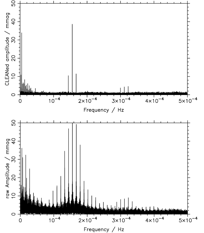
Fig. 2. Power spectrum of the SuperWASP data of 1SWASP J050634.16–353648.4. Lower panel: raw power spectrum, upper panel: CLEANed power spectrum, both with amplitudes in mmag. Strong peaks at frequencies of 1.557 \times 10^{-4} Hz (or 13.45 d -1 ) and 2.268 \times 10^{-6} Hz (or a period around 5.104 d) are seen.
