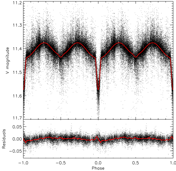
Fig. 8. Eclipsing binary light curve for 1SWASP J050634.16–353648.4, over-plotted with the best-fitting model from PHOEBE. The lower panel shows the residuals between the model fit and the binned data (which we emphasize was not used in the modelling). Around ingress to, and egress from, the primary eclipse, the rapid changes are not as well sampled by the SuperWASP data as in the out-of-eclipse regions, and so give rise to slightly higher residuals of order 0.01 mag.
