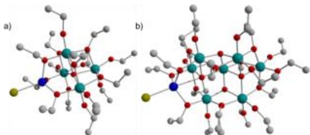
Figure 5. The structures of (a) [Ti 4 O(OEt) 15 CoX] ( 2-X , X = Cl, Br) and (b) [Ti 7 O 5 (OEt) 19 CoX] ( 3-X , Cl, Br). Teal = Ti, red = O, grey = C, blue = Co, green = X.
