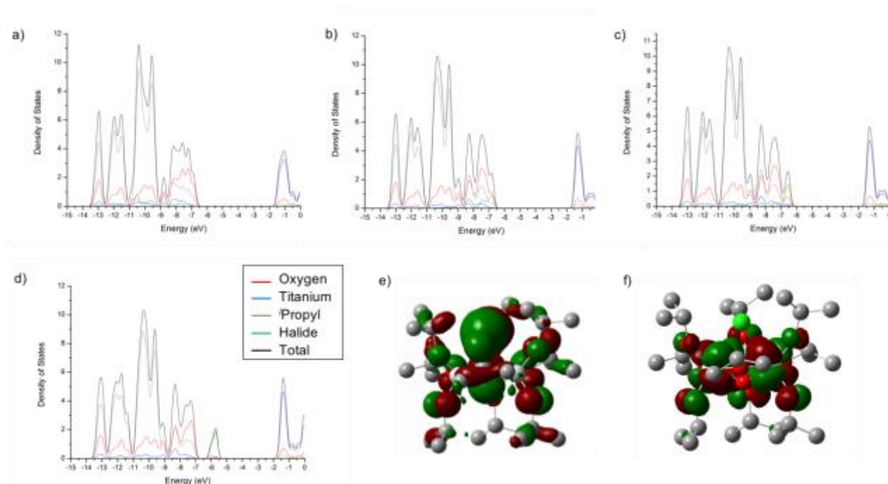
Figure 3. Density of states (DOS) plots for [\text{Ti}_3\text{O}(\text{O}'\text{Pr})_3\text{X}] ( 1\text{-X} ), \text{X} = \text{F} (a), \text{Cl} (b), \text{Br} (c), \text{I} (d) and visualisation of the highest occupied (e) and lowest unoccupied (f) molecular orbitals of [\text{Ti}_3\text{O}(\text{O}'\text{Pr})_3\text{Cl}] (isovalues: \pm 0.02 ). Calculated at the B3LYP/6-31g** (6-311g** for iodine) level of theory.
