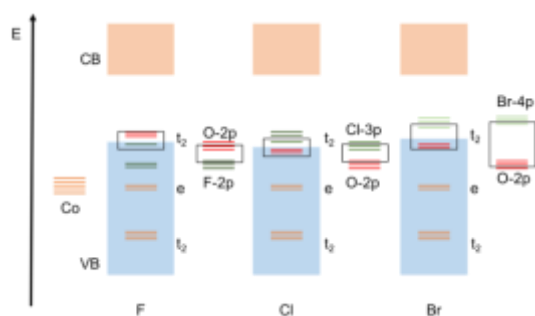
Figure 8. Qualitative molecular orbitals to explain the observed band gap trends in cages 2-X and 3-X. Orange = Co, red = O and green = halide.
