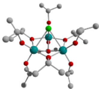
Figure 1. Structure of [\text{Ti}_3\text{O}(\text{O}^i\text{Pr})_9\text{Cl}] ( 1-Cl ). Note the \text{C}_{3v} symmetry of the molecule. Hydrogen atoms are omitted for clarity. Teal = Ti, red = O, grey = C, green = Cl.
