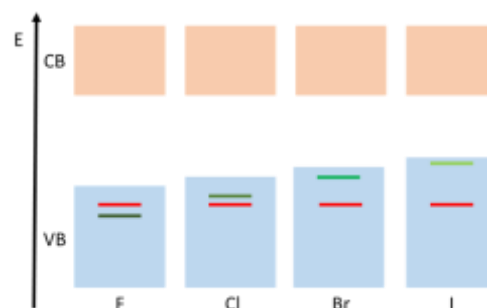
Figure 4. Qualitative diagram demonstrating the influence of the halide on the valence band in the 1\text{-X} ( \text{X} = \text{F}, \text{Cl}, \text{Br}, \text{I} ) family. Red = oxygen contribution, green = halide contribution.
