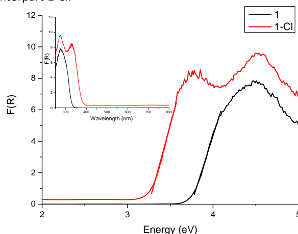
Figure 2. Diffuse reflectance UV-vis spectrum of 1 and 1-Cl . The band gap was determined by the DE method as 3.74 eV for 1 and 3.22 eV for 1-Cl .
