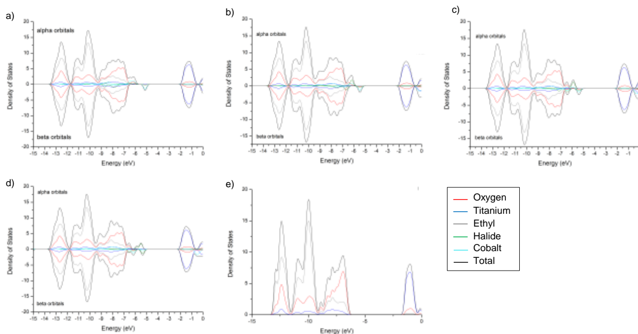
Figure 7. Density of states (DOS) plots for [\text{Ti}_7\text{O}_5(\text{OEt})_{19}\text{CoX}] ( 3-X ), X = \text{F} (a), \text{Cl} (b), \text{Br} (c), \text{I} (d) and (e) the 'undoped' POT cage [\text{Ti}_7\text{O}_5(\text{OEt})_{20}] . Calculated on a B3LYP/6-31g* (6-311g* for iodine) level of theory.
