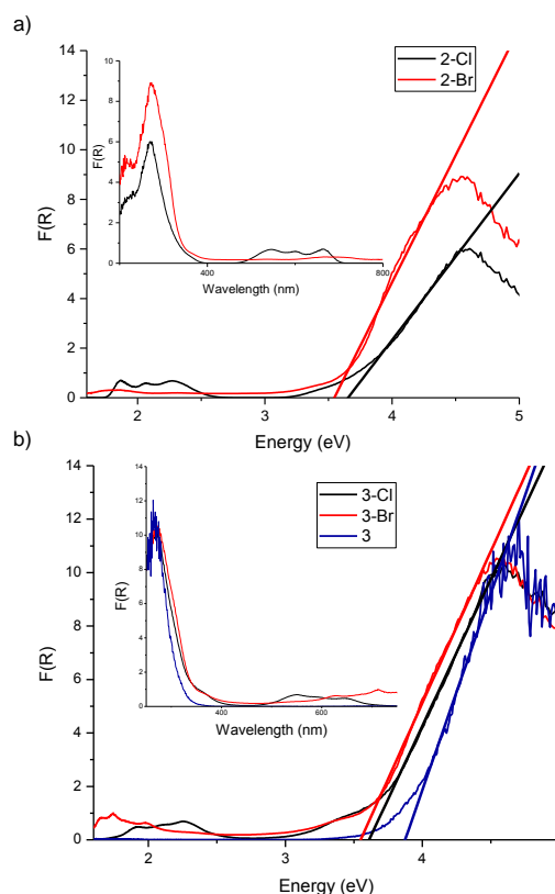
Figure 6. Diffuse reflectance UV-vis spectra of solid (a) [Ti 4 O(OEt) 15 MX] [ 2-X , X = Cl (black), Br (red)] and (b) [Ti 7 O 5 (OEt) 19 CoX] [ 3-X , X = Cl (black), Br (red) and ‘undoped’ 3 (blue)]. The DE method was used in all cases.
