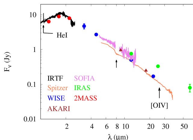
Figure 2. IRTF, Spitzer IRS and SOFIA FORCAST spectra of T CrB, with 2MASS, WISE , AKARI and IRAS photometry superimposed; errors in 2MASS, WISE , AKARI and IRAS photometry are smaller than points if not visible. The He I \lambda = 1.083 \mu\text{m} line is labelled, as is the expected location of the [OIV] \lambda = 25.89 \mu\text{m} line. The arrow at 8 \mu\text{m} shows the SiO absorption feature discussed in Section 8.1.
