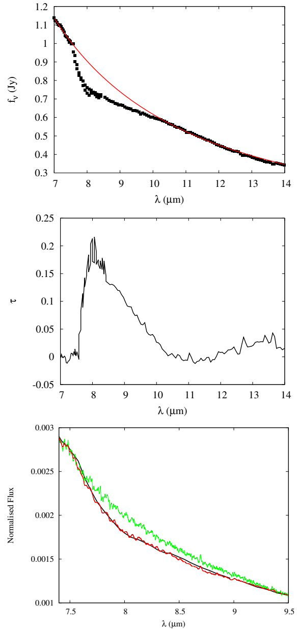
Figure 5. Top: Power-law fit to the continuum around 8 \mu\text{m} as discussed in text. Middle: Optical depth in SiO feature. Bottom: 8 \mu\text{m} feature in T CrB (black). Green curve is contribution of photospheric SiO. Red curve is the combined effect of absorption by SiO in the RG photosphere, with an additional contribution from SiO in the RG wind. The SiO column density is 2.9 \times 10^{17} \text{ cm}^{-2} , the wind temperature is 1,000 K. See text for details.
