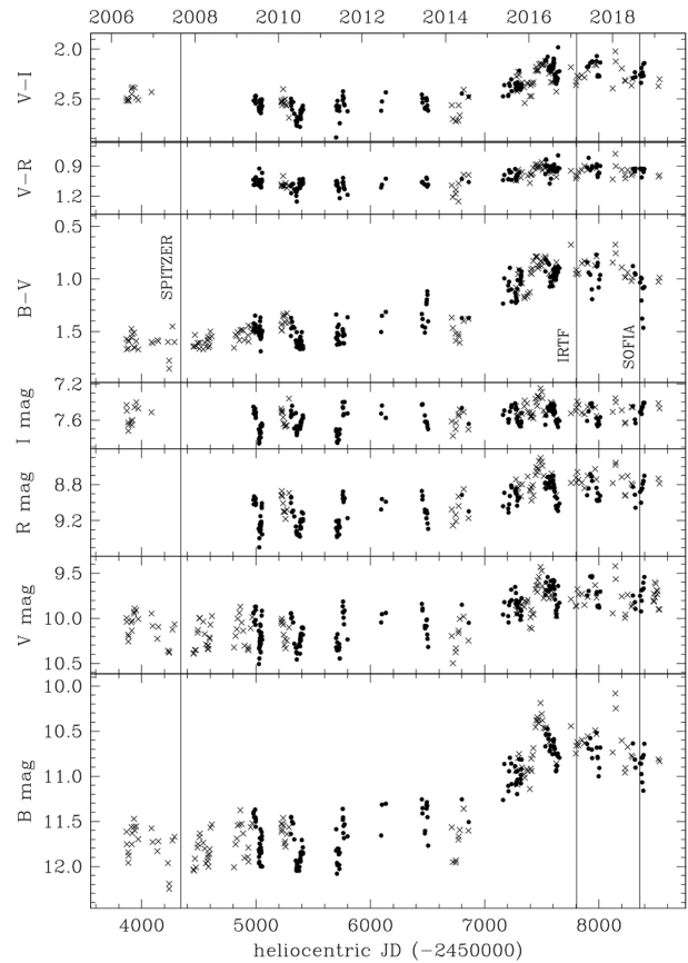
Figure 1. BVRI light curves of T CrB covering the Spitzer , IRTF and SOFIA observations; the JD times of the Spitzer , IRTF and SOFIA observations are indicated. Data from the ANS Collaboration; the different symbols represent data from two separate telescopes, working independently to provide an independent check.
